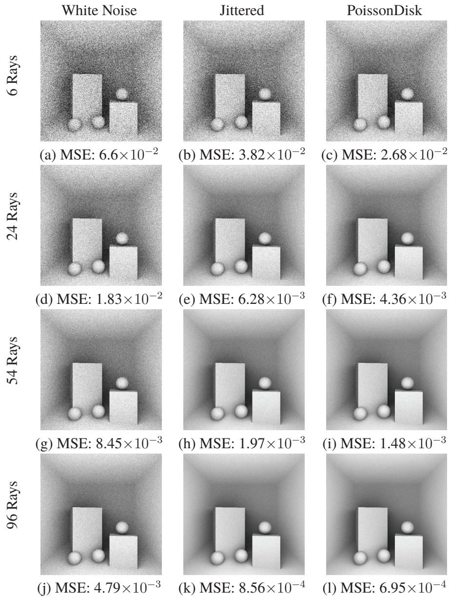
Figure 7.5: Cornell box rendered with ambient occlusion. Mean squared error (MSE) values are computed w.r.t a reference image (shown in Fig. 7.7, for White noise (Left) , Jittered sampling (Center) and Poisson Disk (Right) for a given number of shading rays used to sample directions on the visible hemisphere at each hitpoint in the scene.
