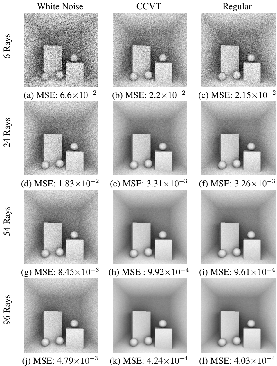
Figure 7.6: Cornell box rendered with ambient occlusion. Mean squared error (MSE) values are computed w.r.t a reference image (shown in Fig. 7.7, for White noise ( Left ), CCVT ( Center ) and Regular Healpix ( Right ) sampling for a given number of shading rays used to sample directions on the visible hemisphere at each hitpoint in the scene.
