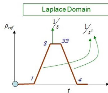
FIGURE 9.20 – Illustration of the internal model construction.
