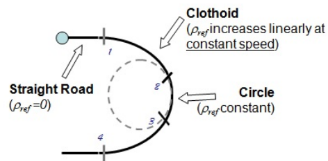
FIGURE 9.19 – modeling of the road geometry.
