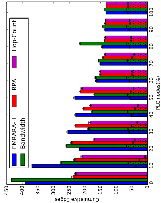
(c) 100 Nodes
