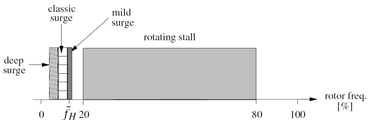
Figure 1-27 Frequencies of several types of aerodynamic flow instabilities with scaled Helmholtz frequency (78)
