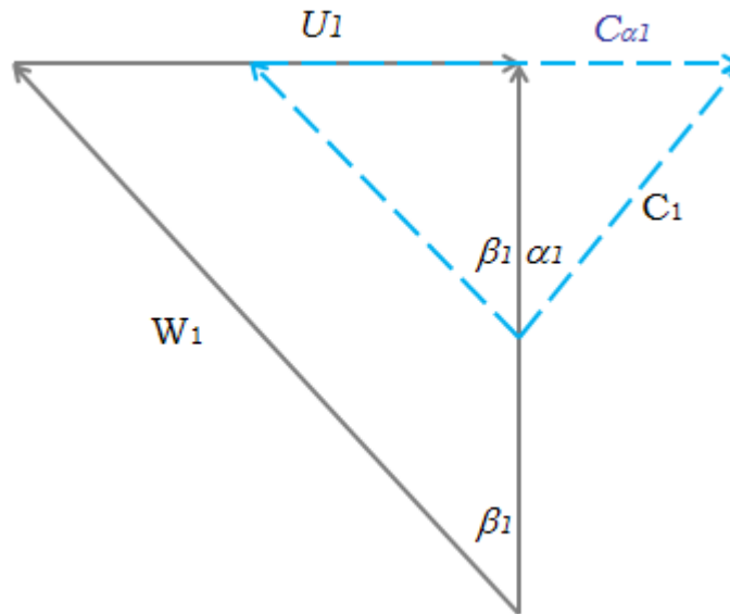
Figure 1-31 Inlet velocity diagram showing reduction in inlet velocity due to positive swirl (71).
