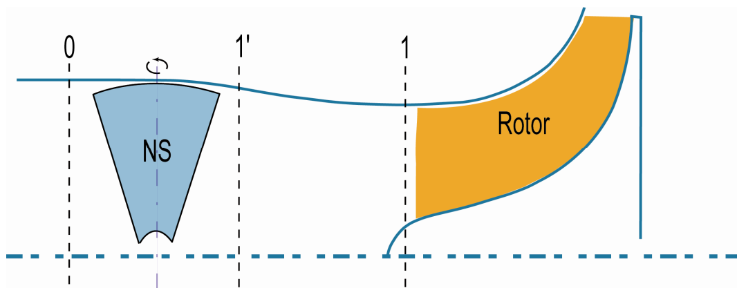
Figure 4-44 New system guide vane
