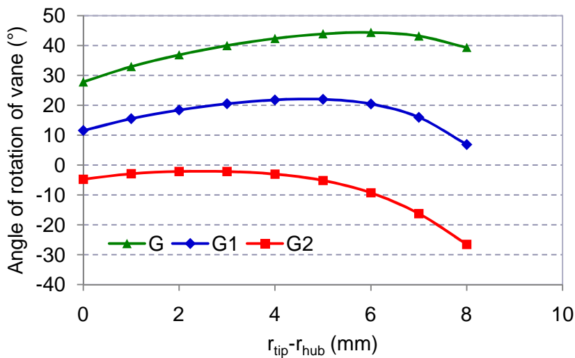
Figure 4-4 Ideal guide vane at constant mean flow rate and 3 different rotational speeds
