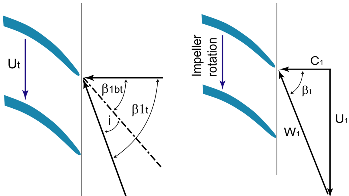
Figure 1-9 Velocity triangle with no swirl at the impeller inducer tip [to the left], and at inducer mean line [to the right]
