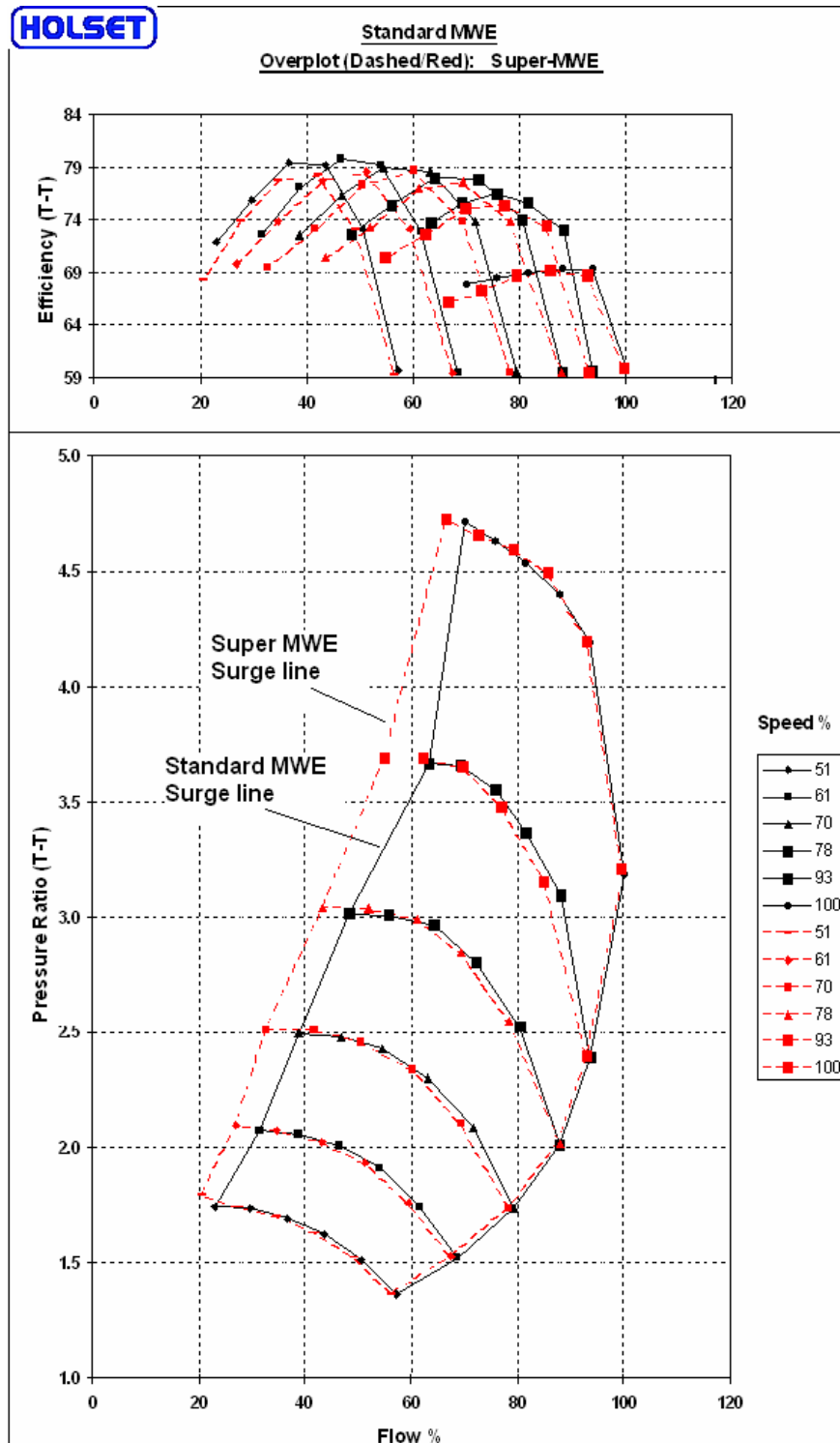
Figure 1-52 Super-MWE compared to conventional MWE (112)
