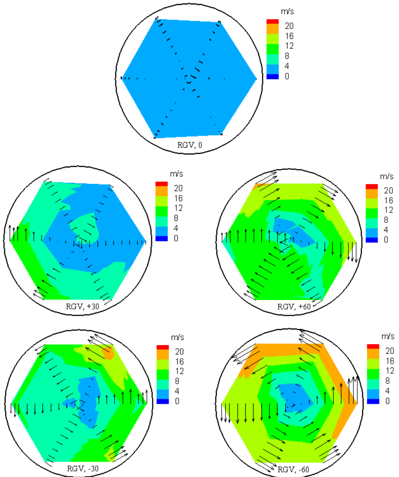
Figure 4-41 Tangential velocity distribution downstream of the RGVs
