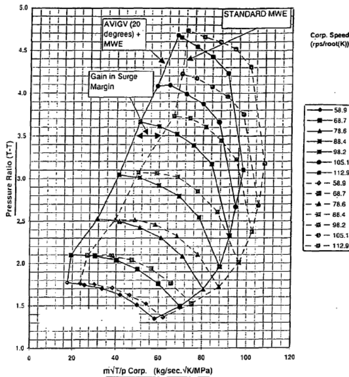
Figure 1-61 Effect on the surge margin using an MWE coupled to AIGVs at +20^\circ (149)
