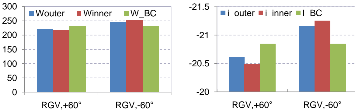
Figure 4-42 Incidence angle [i] and relative velocity [W] calculated for point of the surge limit at N=140K rpm, line with negative and positive RGV vanes angle.
