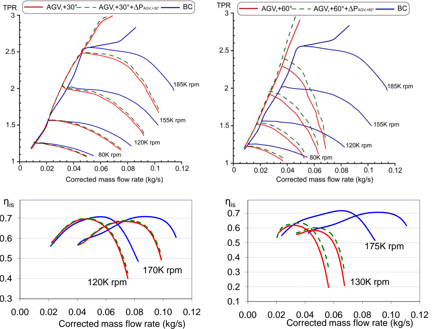
Figure 4-23 Reconstructed pressure and efficiency curves after subtracting pressure losses through the AGVs, for setting angles, \theta = +30^\circ; +60^\circ
