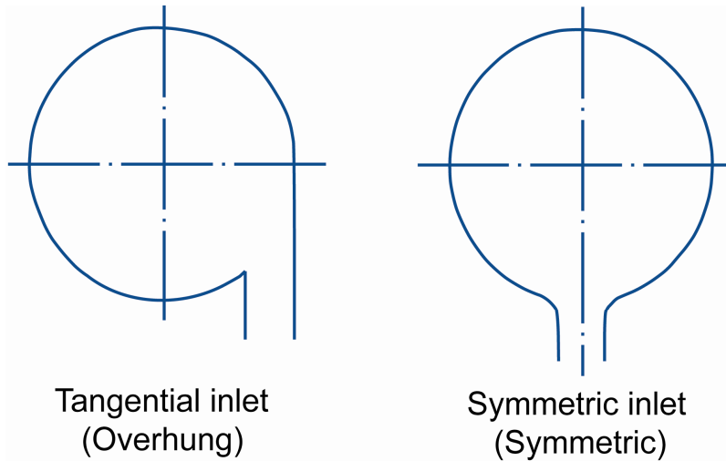
Figure 1-16 Overhung and symmetric volutes
