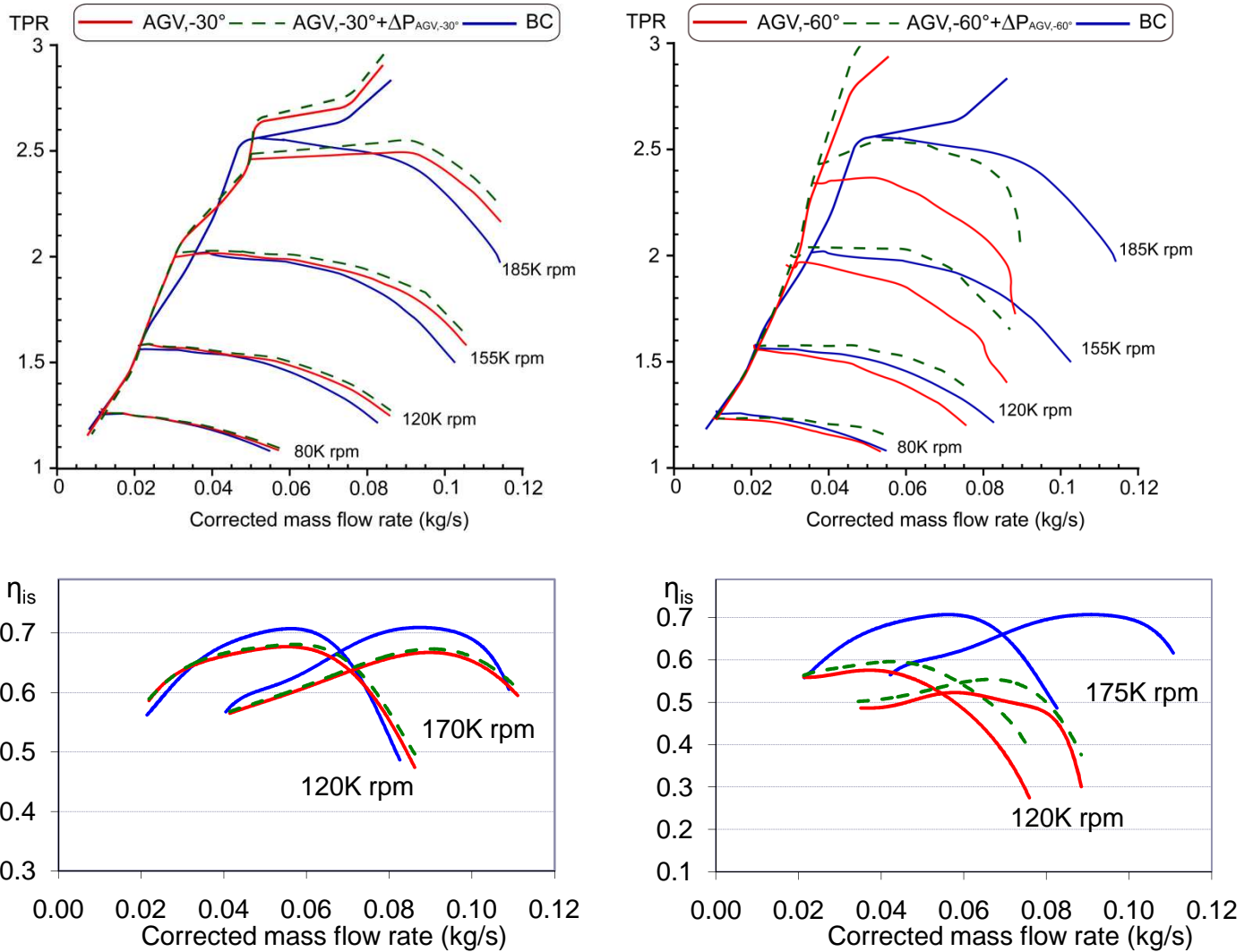
Figure 4-24 Reconstructed pressure and efficiency curves after subtracting pressure losses through the AGVs, for setting angles, \theta = -30^\circ; -60^\circ
