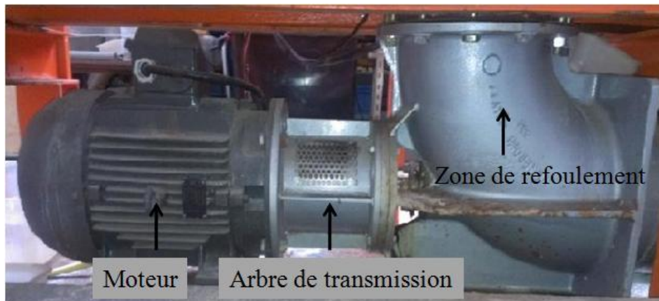
Figure II.2 : Pompe hélice
