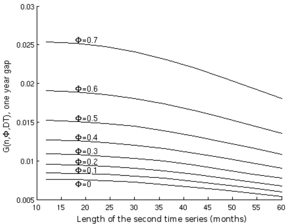
Figure 7: Effect of the length of the second time series on the uncertainty trend coefficient G , Eq.(15) with (a) a one year overlap and (b) a one year gap.
