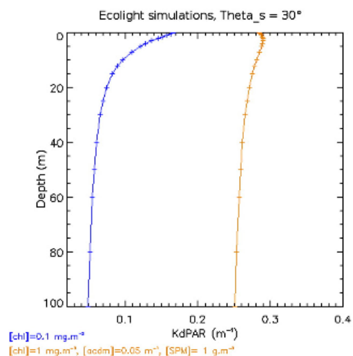
Fig. 1. Simulated K_{dPAR}(z) in the water column using Ecolight for clear water with low [Chl- a ] (case 1, blue) and coastal water (case 2, orange). (For interpretation of the references to colour in this figure legend, the reader is referred to the web version of this article.)
