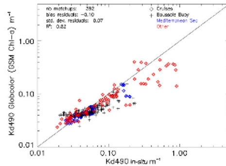
Fig. 3. Morel's K_{d490} vs. in-situ.
