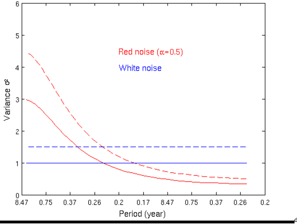
Figure 9: Theoretical Fourier spectrum, Eq. (21), as a function of the period for a white noise (blue curve) and a red noise (red curve), this latest being representative of a geophysical time series. In dashed lines the corresponding 95% confidence levels, Eq.(20)
