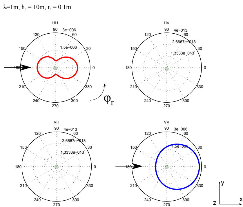
FIGURE 7.2: Scattering coefficients varying with \varphi_r for the cylinder alone with incidence perpendicular to the cylinder axis. The direction of incidence is shown by the black arrow.
