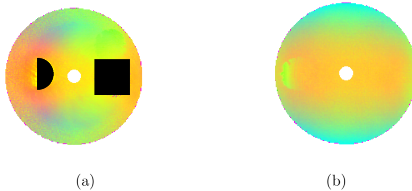
FIGURE 5.13: RGB color channel visualization issued from the Kennaugh matrix equivalent to the Mueller measured matrices.
