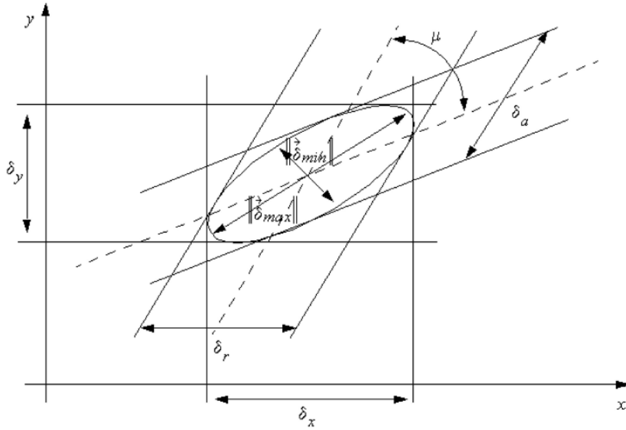
FIGURE 1.11: The resolution ellipse can be defined by several preferred directions, extracted from [15].
