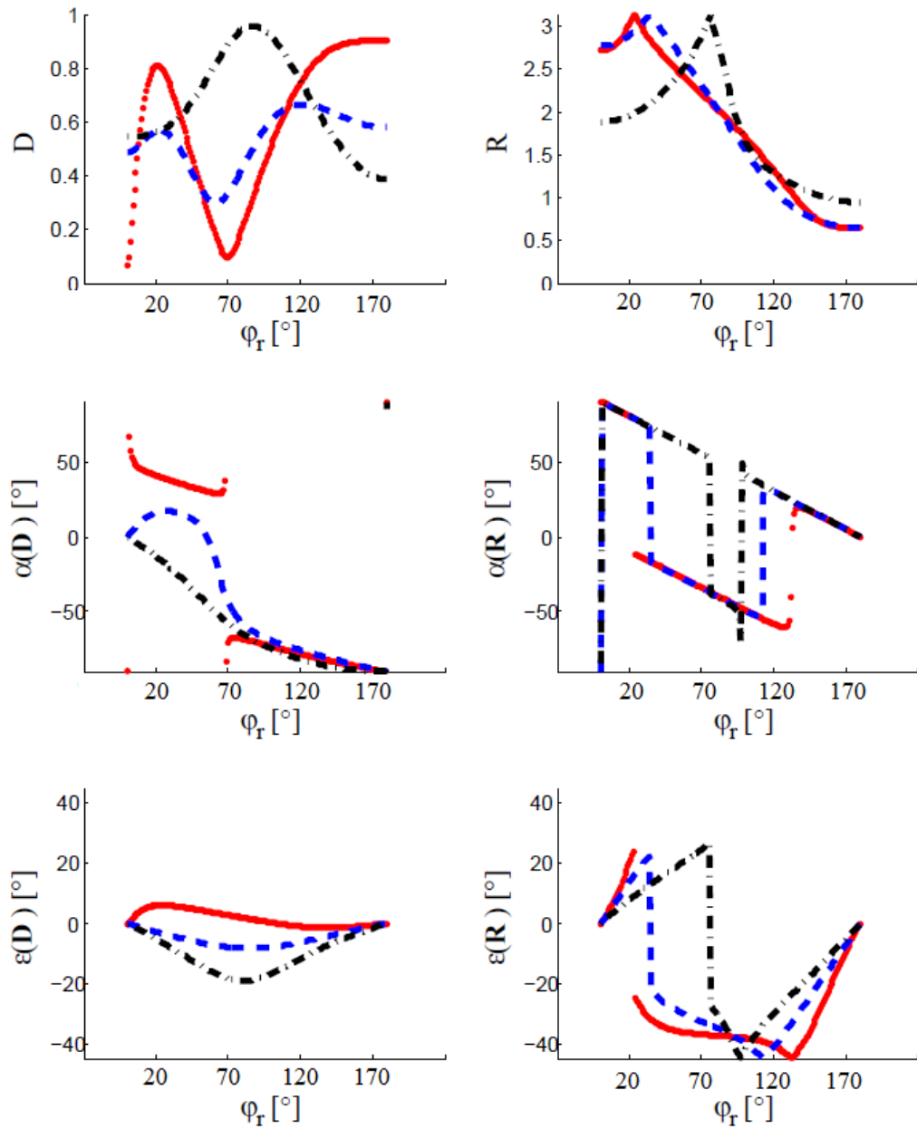
FIGURE 7.12: Study of the influence of \varepsilon_e on decomposition parameters R and D varying with \varphi_r Legend: red \varepsilon_e = 12 - 0.3j , in dashed blue \varepsilon_e = 12 - 3j , in dotted black \varepsilon_e = 12 - 30j .
