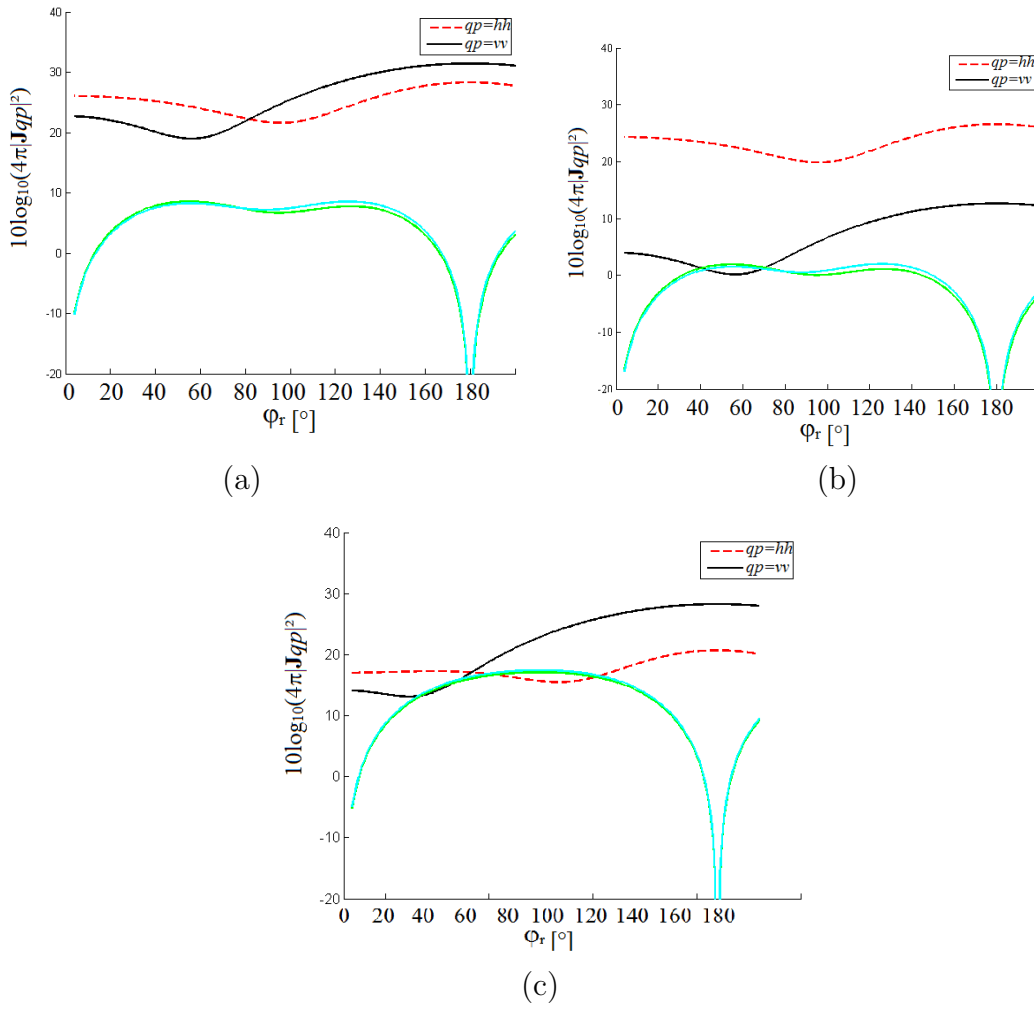
FIGURE 7.10: Scattering coefficients of a single dielectric cylinder taking into account the ground interactions. (a) \theta_e = 70^\circ and metallic ground, (b) \theta_e = 70^\circ and \epsilon_e = \epsilon_{ground} , (c) \theta_e = 35^\circ and metallic ground.
