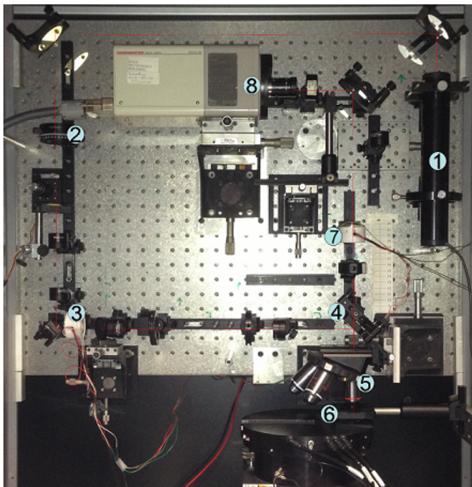
FIGURE 4.8: Picture of the optical setup for the Angle Resolved Polarimeter. 1: laser source; 2: diffuser; 3: PSG; 4: splitter; 5: objective; 6: sample; 7: PSA; 8: camera
