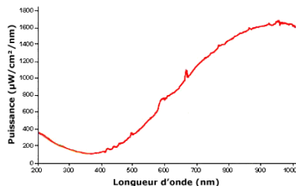
FIGURE 5.1: Emission spectra of the original white source
