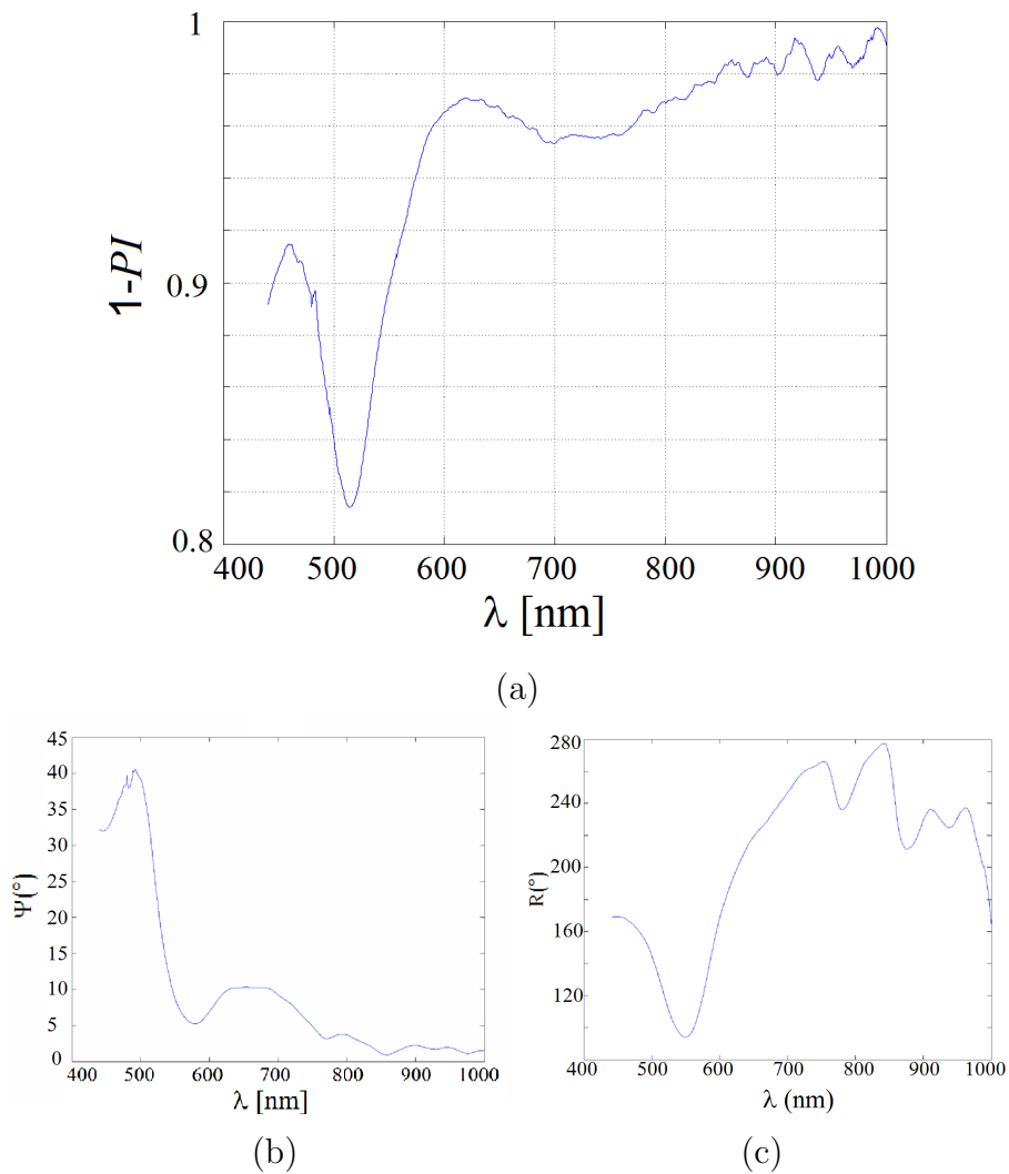
FIGURE 4.7: Lu & Chipman decomposition applied to the spectroscopic measurement on lithographed Carbon Nanotube sample at 60° of incidence in the specular direction. (a) the PI, (b) \Psi [0° – 45°] which is related to the diattenuation via D = \cos(2\Psi) , and (c) the retardance R [80° – 280°].
