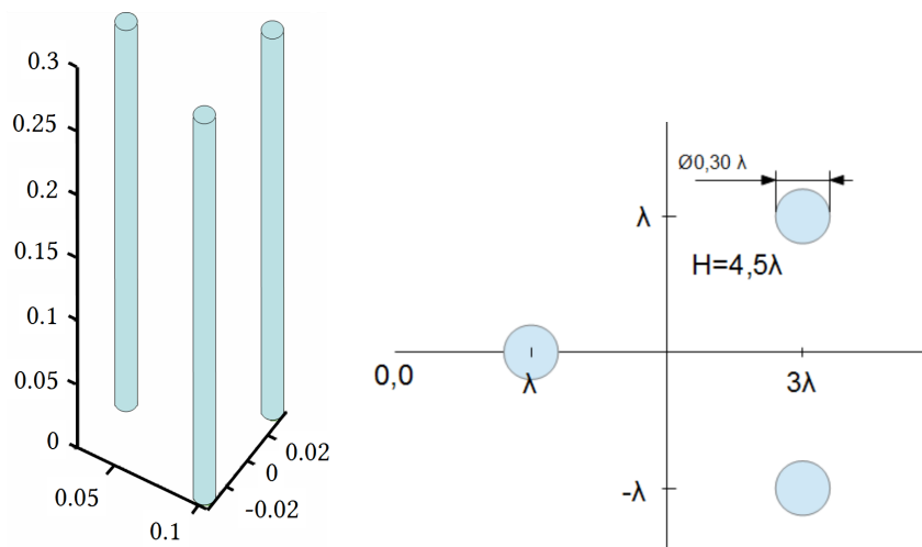
FIGURE 6.8: Configuration of the cylinders for the validation of the simulation code
