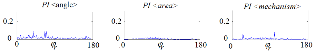
FIGURE 7.19: Comparison of the depolarization index PI for three averaging methods. \theta_r = \theta_e = 40^\circ , \varphi_r = 0^\circ, 180^\circ , \varphi_e = 0^\circ .
