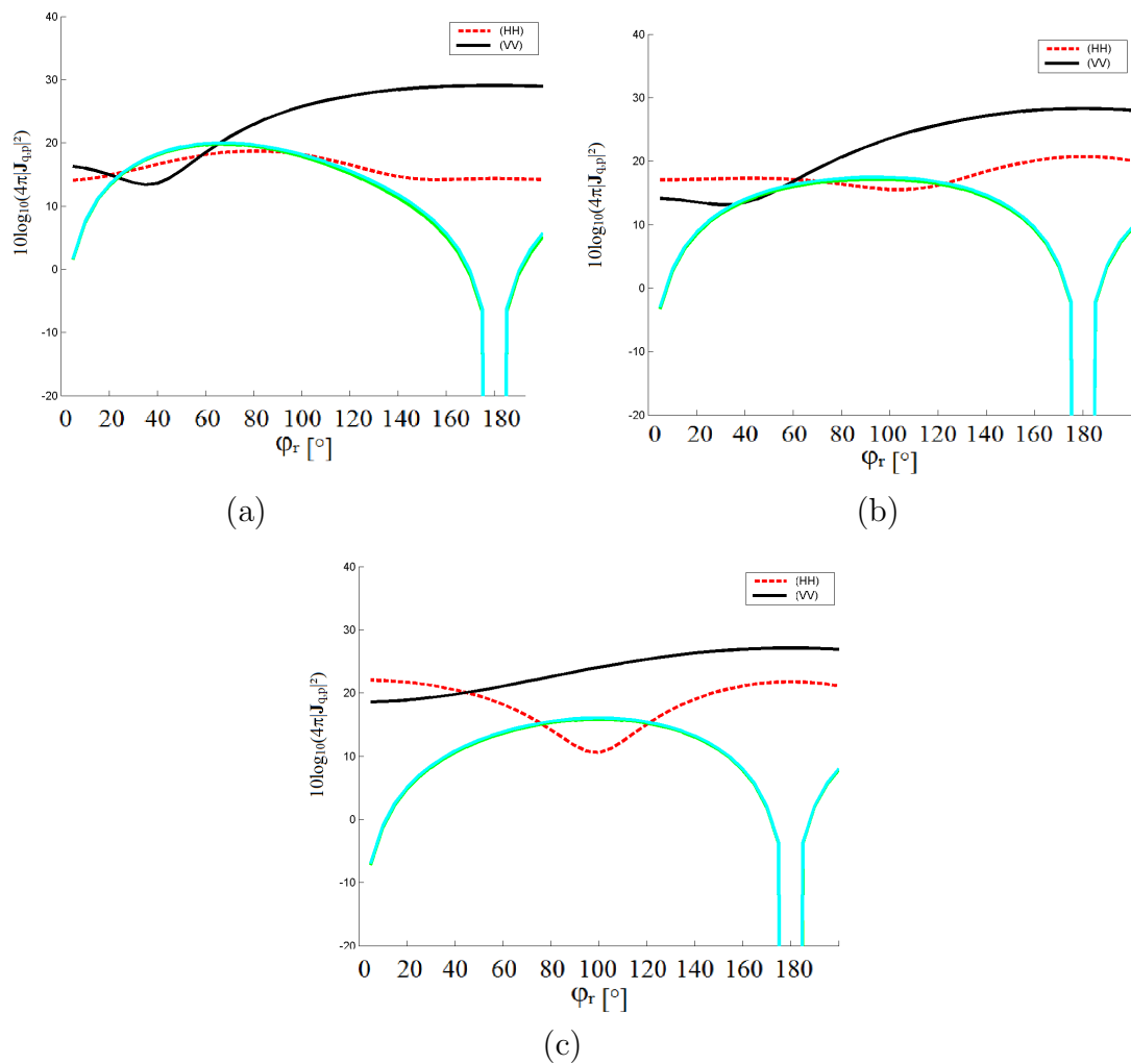
FIGURE 7.11: Study of the influence of \varepsilon_e on the scattering coefficients of the single cylinder varying with \varphi_r . (a) \varepsilon_e = 12 - 0.3j , (b) \varepsilon_e = 12 - 3j , (c) \varepsilon_e = 12 - 30j . Legend: black line: vv polarization, dashed red hh polarization, cyan line hv polarization, green line vh polarization.
