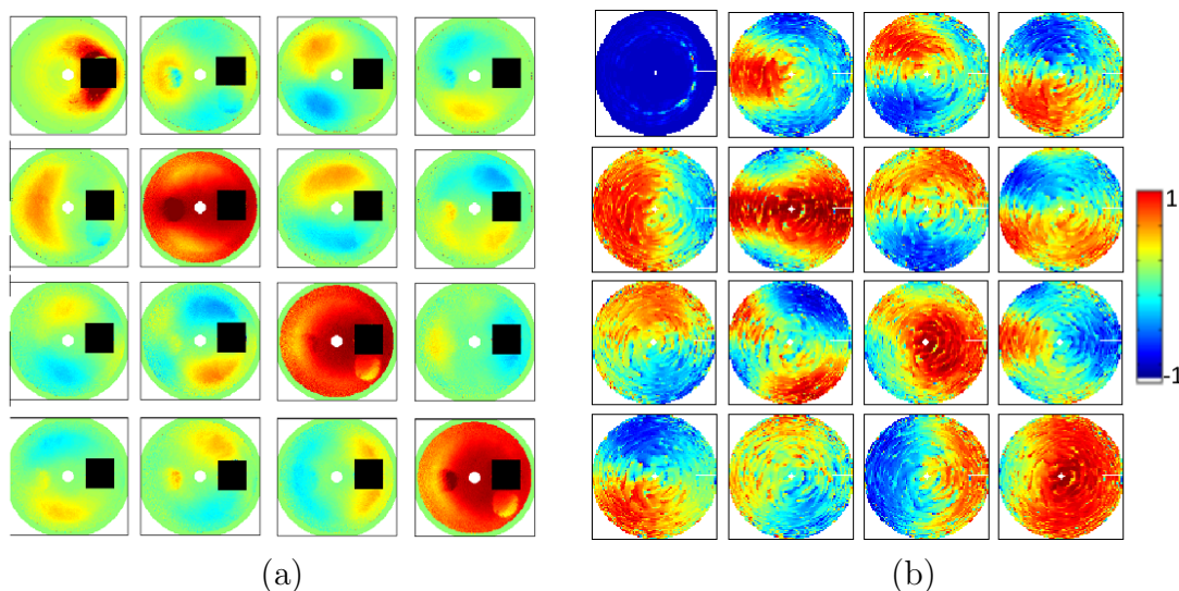
FIGURE 6.12: (a) Sparse forest measurement , (b) Conoscopic normalized Mueller matrix for the simulated Carbon Nanotube Forest for sparse distribution. \mathbf{M}_{1,1} = 1 is replaced by the total intensity
