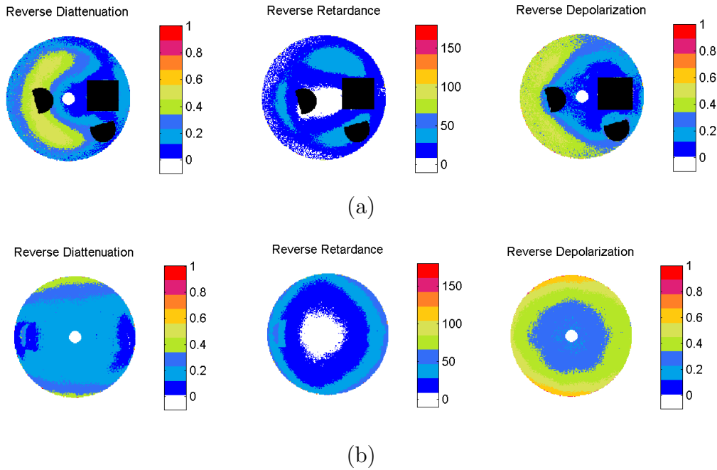
FIGURE 5.11: Reverse Lu Chipman decomposition for two densities of measured forests. (a) the sparse forest, and (b) the dense forest.
