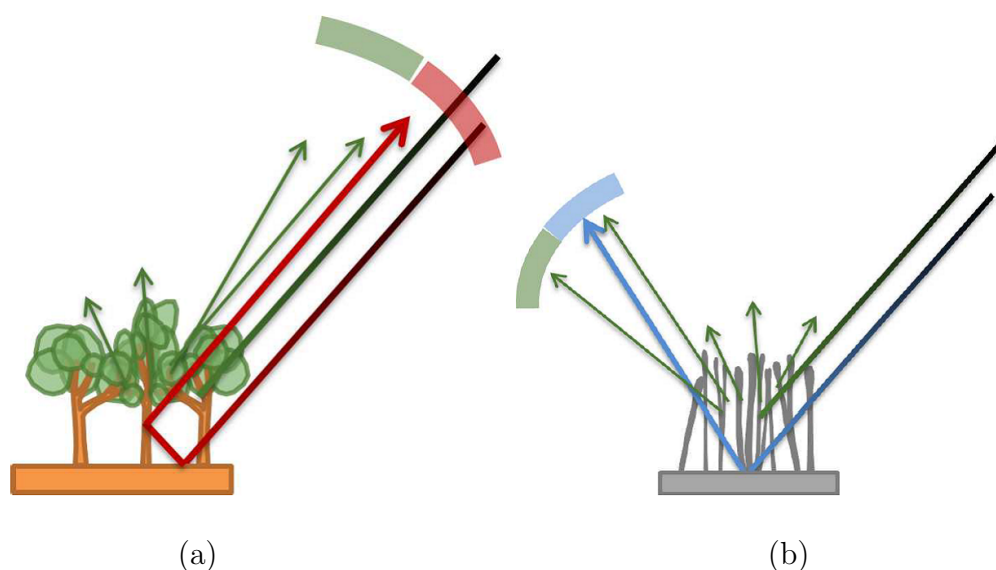
FIGURE 4.4: Backscattering radar (a) or specular optical (b) scattering configuration by the ground, or double bounce on the ground and the trunks, hide the depolarization related to the volume diffusion.
