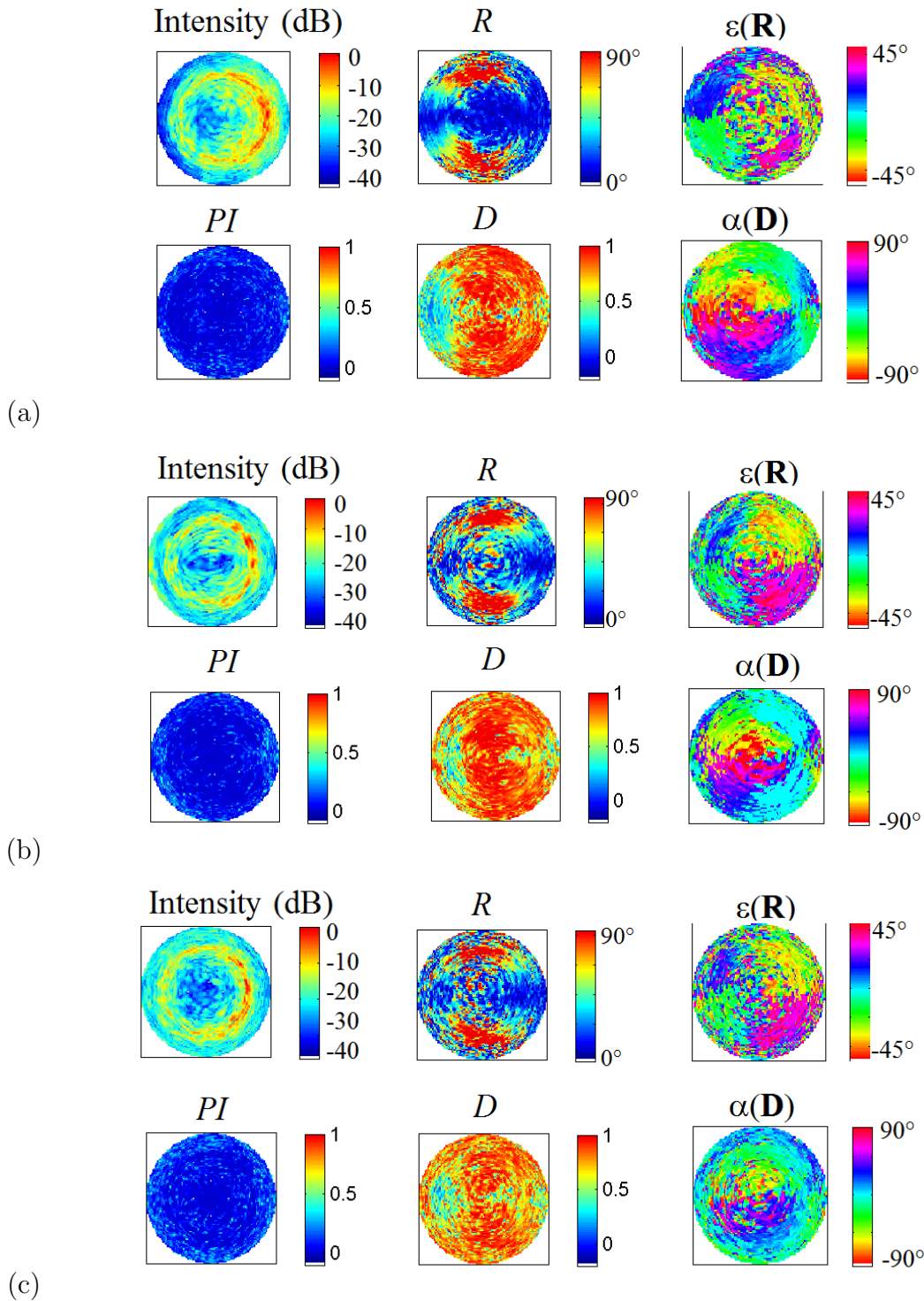
FIGURE 8.5: Lu and Chipman decomposition applied on the three types of branch inclinations. (a) horizontal branch orientations (b) 45° horizontal branch orientations, (c) random horizontal branch orientations.
