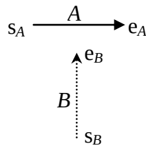
Figure I.4 DRA relations
