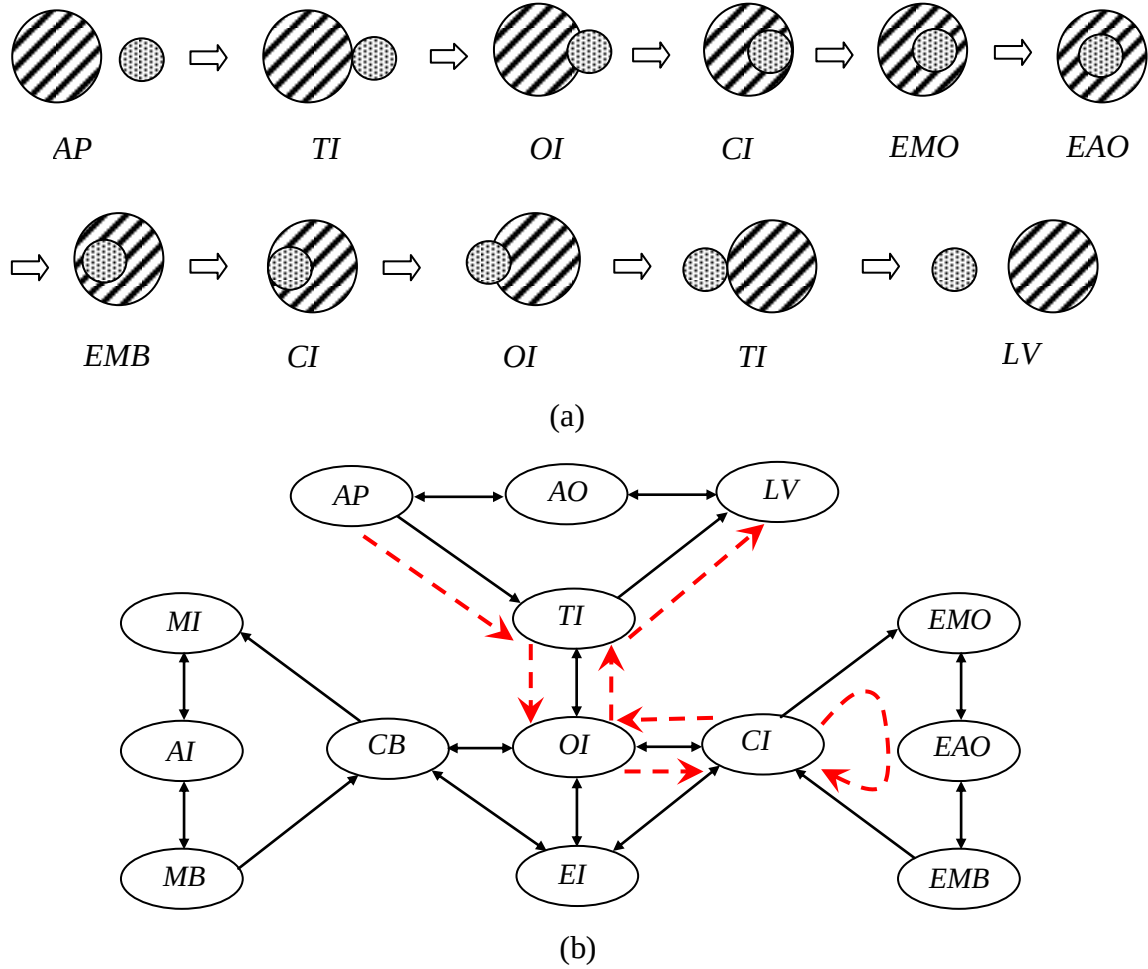
Figure IV.3 Continuous transitions of A moving over a smaller region B
