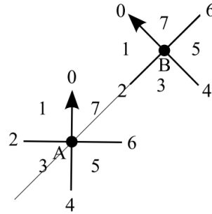
Figure I.5 OPRA 2 relations
