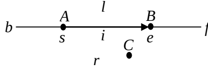
Figure I.3 LR relations
