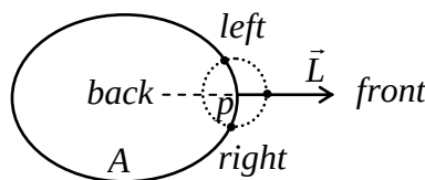
Figure II.4 A neighbouring disc neigh(p)
