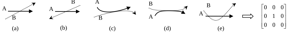
Figure II.10 Some Cross/touch relations that cannot be distinguished by the HBT model
