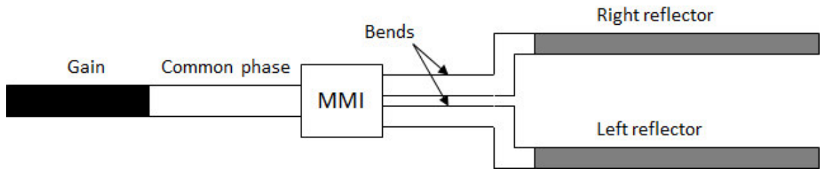
Figure 63- Structure of the modulated grating Y laser
