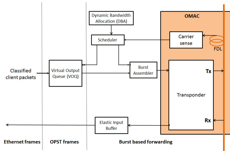
Figure 21- Functional blocks of an OPST node
