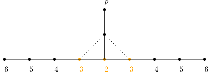
FIGURE 10.1. The type p is determined by three vertices in the infinite branch.
