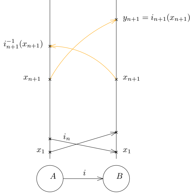
FIGURE 2.3. The back-and-forth argument
