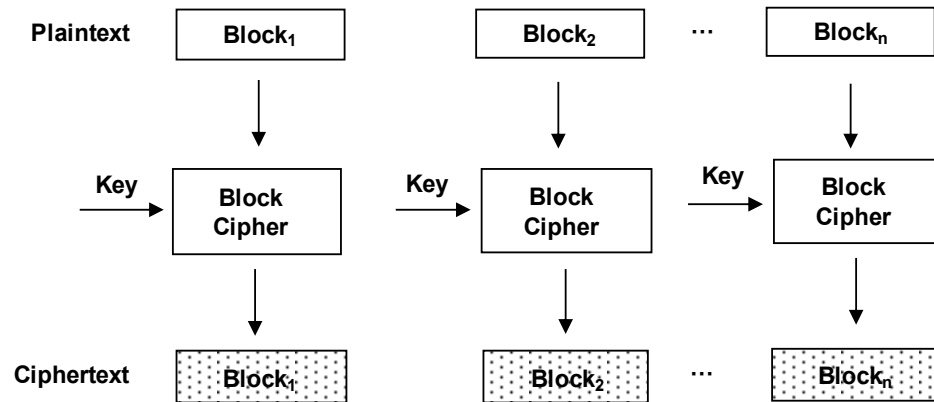
Figure 4. Electronic Codebook Mode (ECB)
