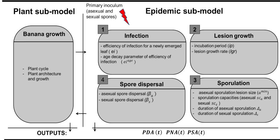
Figure 1: Overview of the host-pathogen model (banana/BLSD) general framework and the articulation of the plant sub-model and the epidemic sub-model. Only parameters of the epidemic sub-model are mentioned. PDA is the percentage of disease area, PNA is the percentage of necrotic area and PSA is the percentage of asexual sporulating area.
