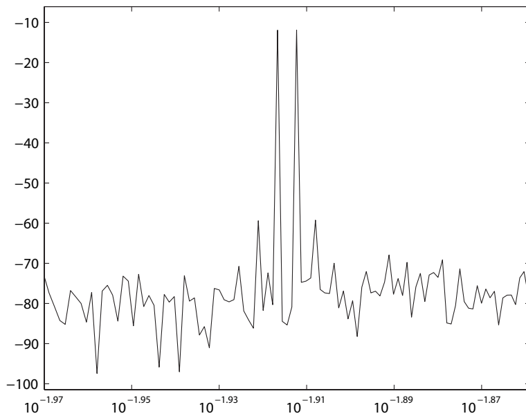
Figure 5.22: Two tone test of the designed modulator. with two sinusoidal inputs at two adjacent frequency 397 Hz and 401 Hz, amplitude at -12 dBFS, IM3 is simulated at 47.3dB.
