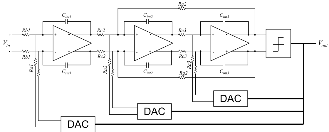
Figure 5.26: The schematic of a differential 3 rd active RC CIBF modulator
