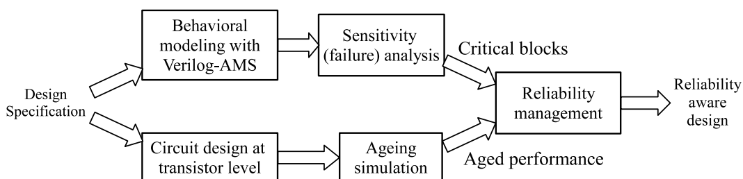
Figure 3.35: The flowchart of ageing managements with hierarchical reliability analysis and block failure estimation.
