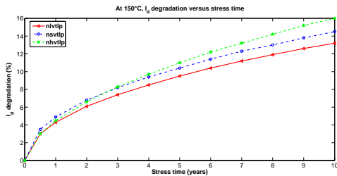
(a) HCI induced I_d degradation at 150^\circ C
