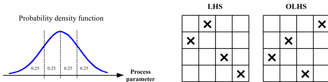
Figure 3.11: Probability density function, LHS, OLHS when sample size = 4.
