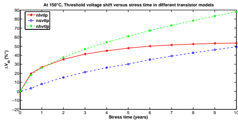
(a) HCI induced V_{th} degradation at 150^\circ C
