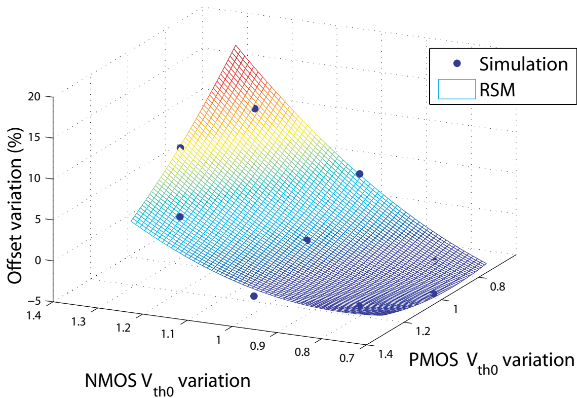
Figure 4.22: The fixed RSM between NMOS/PMOS V_{th0} and comparator offset voltage.
