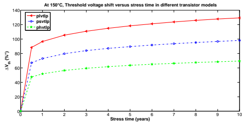
(b) NBTI induced V_{th} degradation at 150^\circ C
