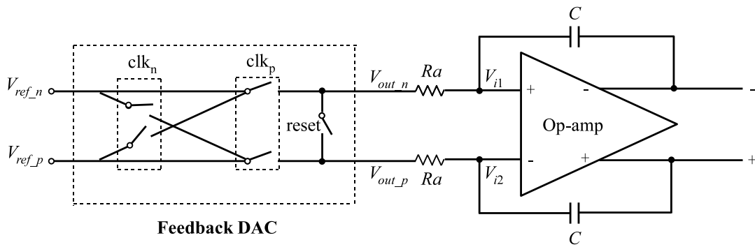
Figure 5.20: Schematic view of 1 bit RZ-DAC, based on transmission gates: Clk_p and Clk_n are generated by the preceding logic. They control the states of the outputs, to be Vref_p - Vref_n or inversely. Reset signal shorts two output ports, making the output return to common mode voltage of the amplifier. In order to avoid short circuit happening, all the switches are closed during a certain same period of the clock edges. Thus, nonoverlapping scheme is employed.
