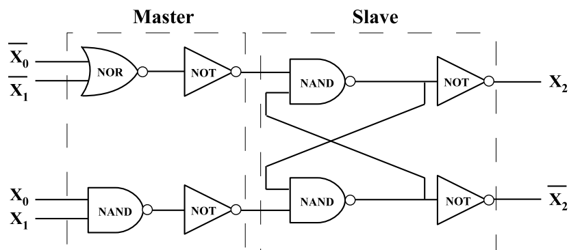
Figure 3.30: The MAS-MRF design structure applied to NAND gate.
