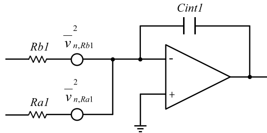
Figure 5.8: Noise calculation with RC integrator model.
