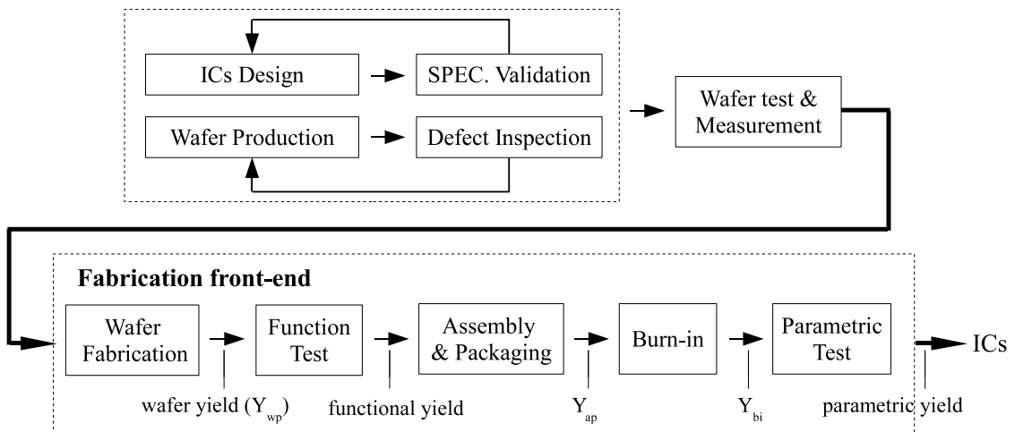
Figure 2.12: The manufacturing process flow of ICs: a perspective of yield in the fabrication fronts-end.
