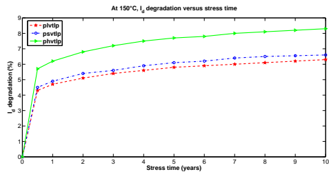
(b) NBTI induced I_d degradation at 150^\circ C
