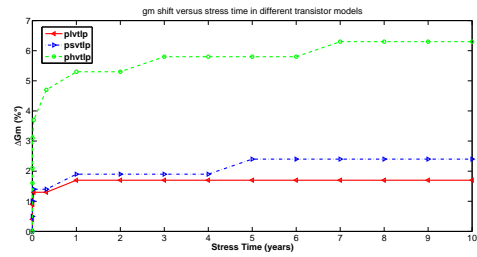
(b) NBTI induced g_m degradation
