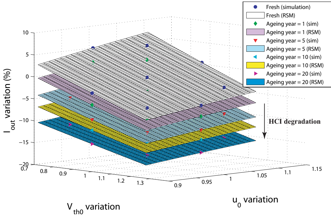
Figure 4.19: Statistical analysis of NMOS current mirror: varied RSMs between BSIM4 parameters and circuit performance.
