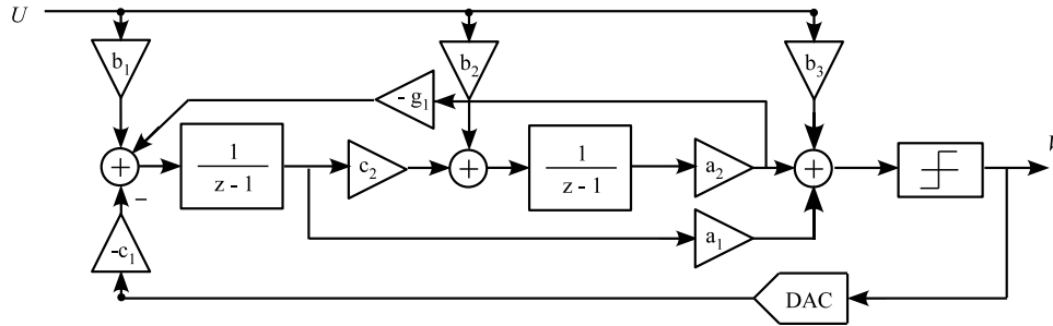
(b) The CIFF loop filter
