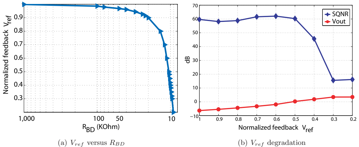
Figure 5.25: A tentative study on TDDB mechanism in \Sigma\Delta modulator. TDDB can influence the feedback reference voltage V_{ref} in DAC.
