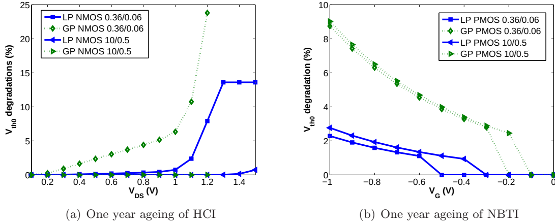
Figure 4.5: Aged transistor performance of LP and GP transistors. GP family transistors are more sensitive to HCl (NMOS) and NBTI (PMOS) than their LP counterparts.
