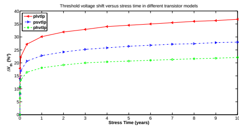
(b) NBTI induced V_{th} degradation
