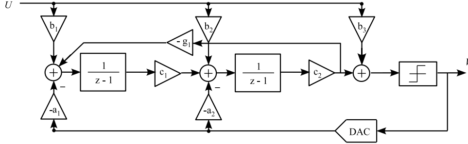
(a) The CIFB loop filter
