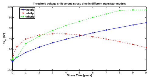
(a) HCI induced V_{th} degradation
