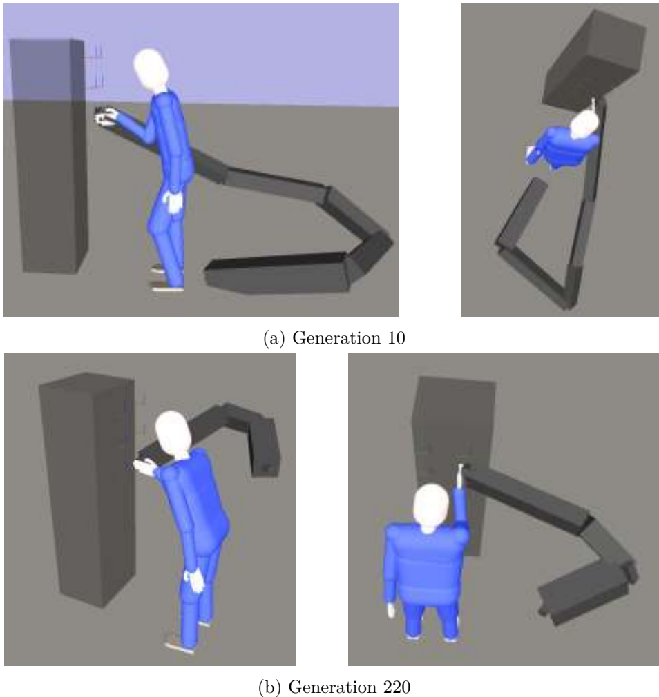
Figure 6.10: Shortest robot of the Pareto front for the 10 th and 220 th generations. Over generations, the overall length of the robot decreases, while the biomechanical solicitations experienced by the worker are kept constant or decreased. The gray cuboid represents the wall where the slab to drill is set (the robot cannot go through this wall).
