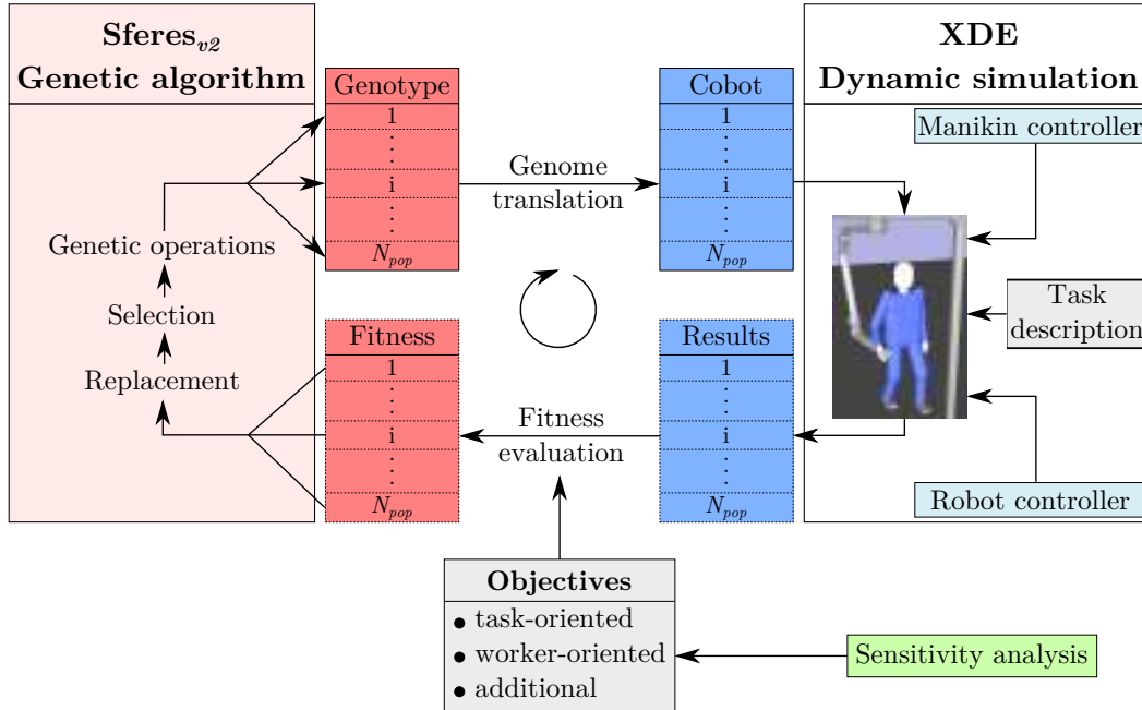
Figure 6.2: Framework for the optimization of cobots design: XDE-Sferes v2 coupling (only one generation loop is represented). The genetic operations are performed by the Sferes v2 software, which provides a population of robot candidates to evaluate. For each candidate, the objectives are measured through an XDE simulation. The objectives include worker-oriented objectives ( i.e. the ergonomic benefit provided by the collaborative robot), task-oriented objectives ( i.e. quality of task execution) and additional objectives ( e.g. cost, complexity...). In order to reduce the overall number of objectives, only the most discriminating ergonomic indicators are included in the worker-oriented objectives (according to the analysis method describes in chapter 5).
