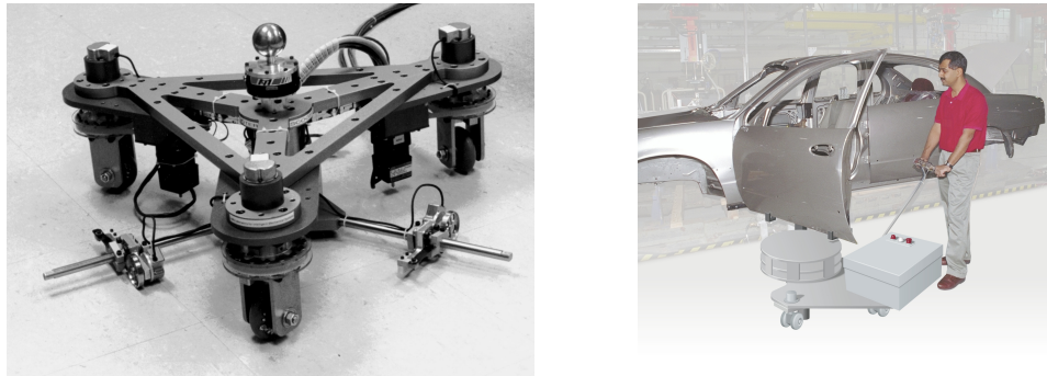
Figure 1.5: Scooter cobot: virtual paths are implemented thanks to the computer-controlled steering of the three wheels, in order to reduce inertia effects in direction changes.
