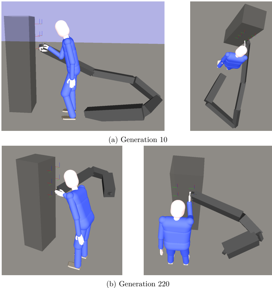
Figure 6.10: Shortest robot of the Pareto front for the 10 th and 220 th generations. Over generations, the overall length of the robot decreases, while the biomechanical demands experienced by the worker are kept constant or decreased. The gray cuboid represents the wall where the slab to drill is set (the robot cannot go through this wall).
