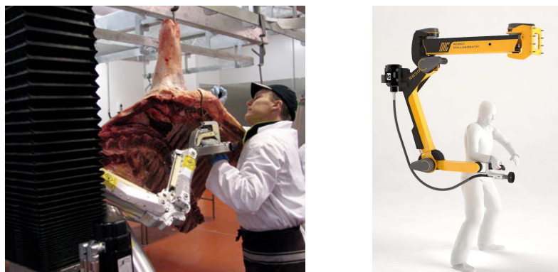
Figure 1.6: Collaborative robots providing strength amplification. Left: HookAssist (Kinea Design) for beef boning. Right: Cobot 7A.15 (RB3D, CEA-LIST, CETIM) for tire retreading or machining.
