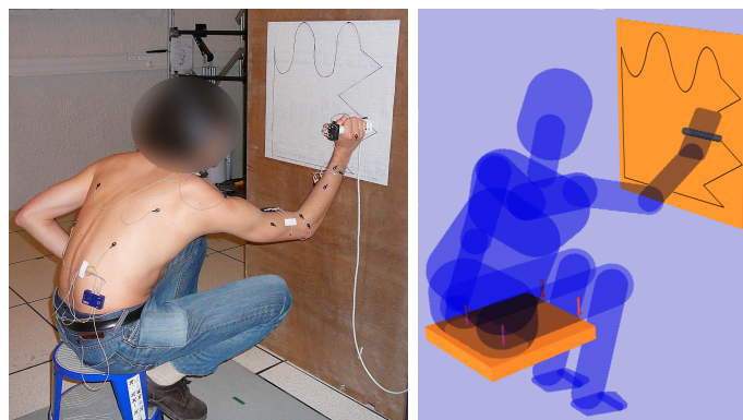
Figure 4.9: Left: A human subject performs the task while his motion and interaction forces are recorded. Right: The motion is replayed with the virtual manikin and the LQP controller.
