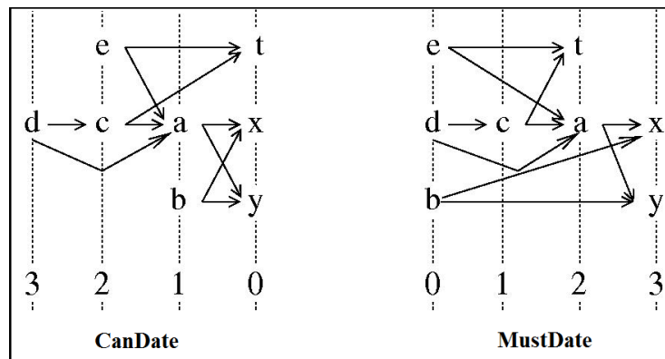
Figure II.11 – CanDate et MustDate
