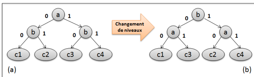
Figure III.11 – Application de l'ordonnancement DVO
