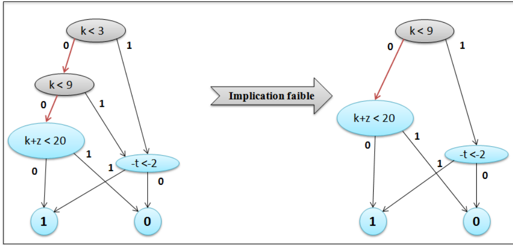
Figure III.10 – Implication faible
