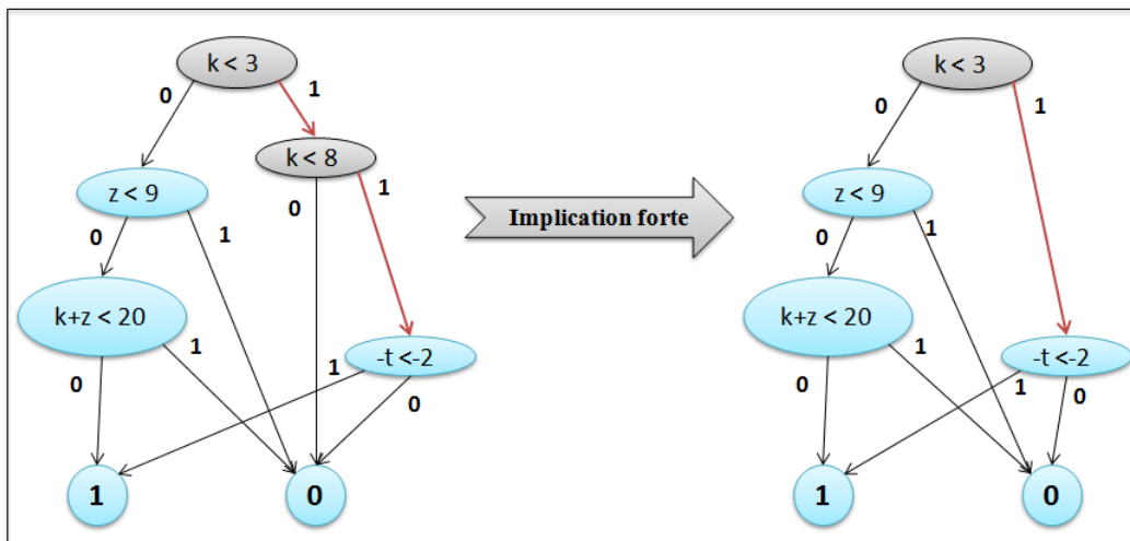
Figure III.9 – Implication forte
