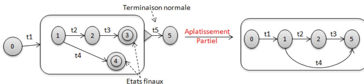
Figure IV.4 – Raccordement d'une transition normale
