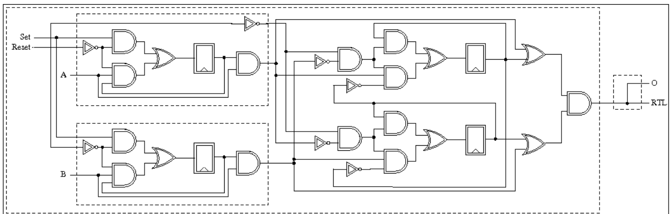
Figure II.10 – Compilation du programme ABO en Light Esterel
