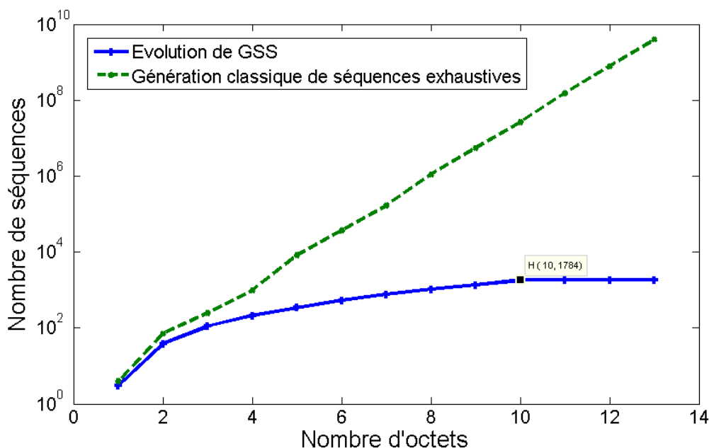
Figure V.10 – Evolution des tests
