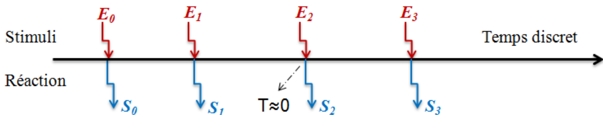
Figure II.3 – Hypothèse synchrone.
