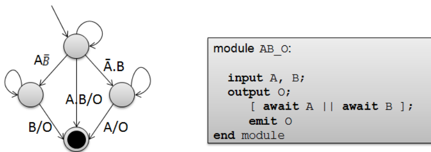
Figure II.6 – Programme ABO.
