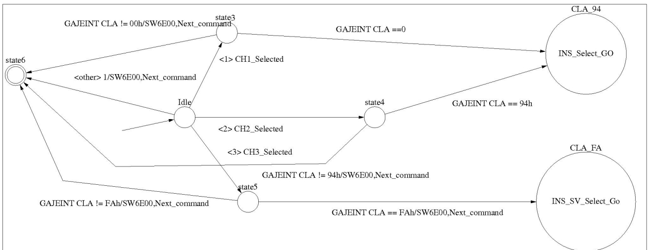
Figure V.5 – Start Command en galaxy
