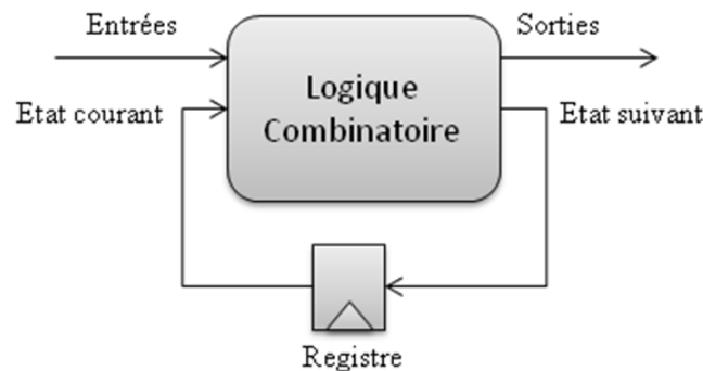
Figure II.7 – Circuit séquentiel synchrone.
