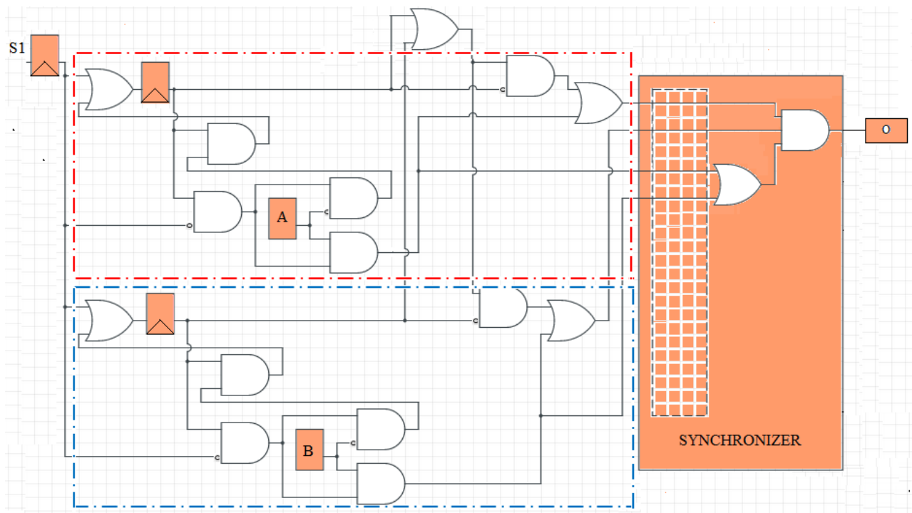
Figure II.8 – Compilation en circuit du programme ABO.
