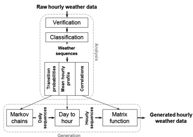
Fig. 1. Sketch of the outdoor climate mathematical model, Runeole.
