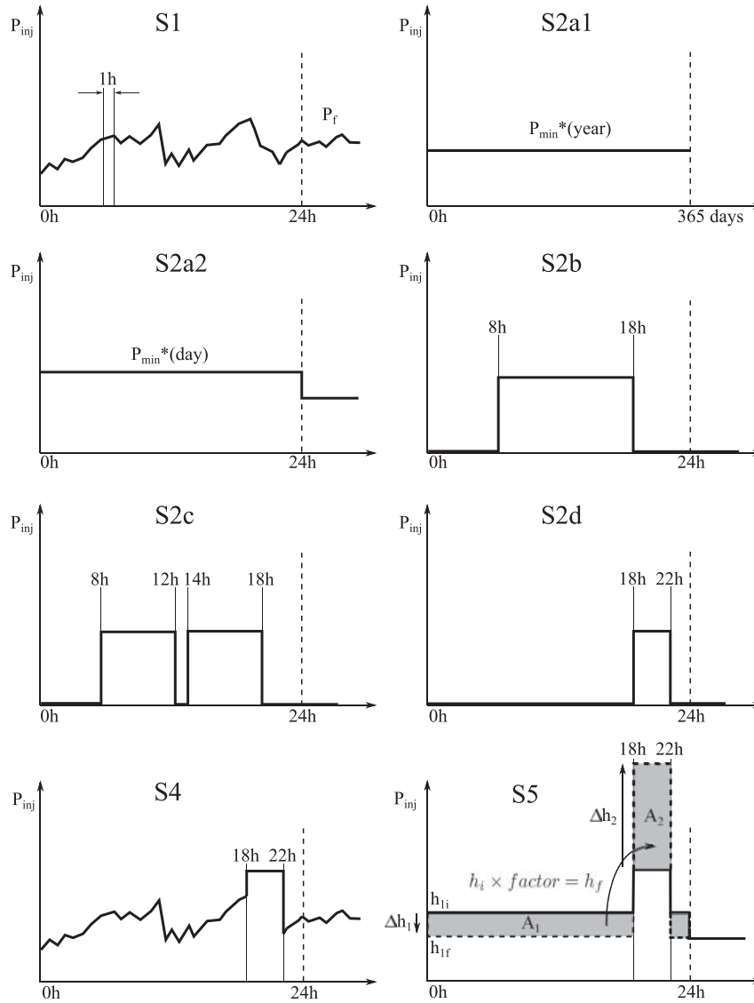
Fig. 3. System services.
