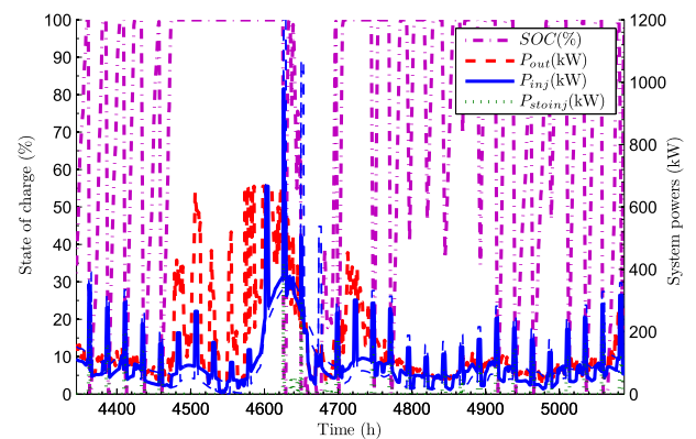
Fig. 12. Simulation results for service S4 (July 2006).
