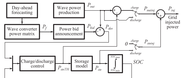
Fig. 5. Modeling block diagram.
