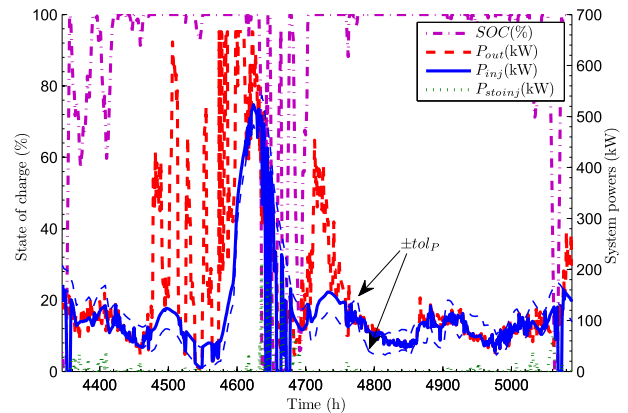
Fig. 7. Simulation results for service S1 (July 2006).
