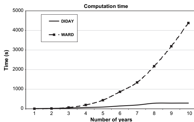
Fig. 2. Computation time of the two automatic classification methods.
