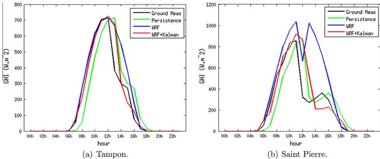
Fig. 11. GHI forecasted and measured for one day.
