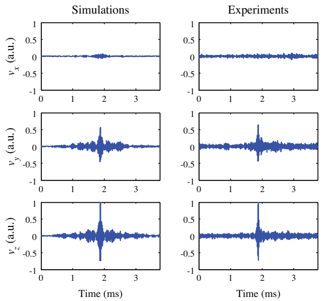
Fig. 3. Time histories of the velocity components at the focal point, for the problem settings described in Fig. 2. Simulated (left column) and experimental (right column) results. For each column, data are normalized with respect to the peak amplitude of v_z .
