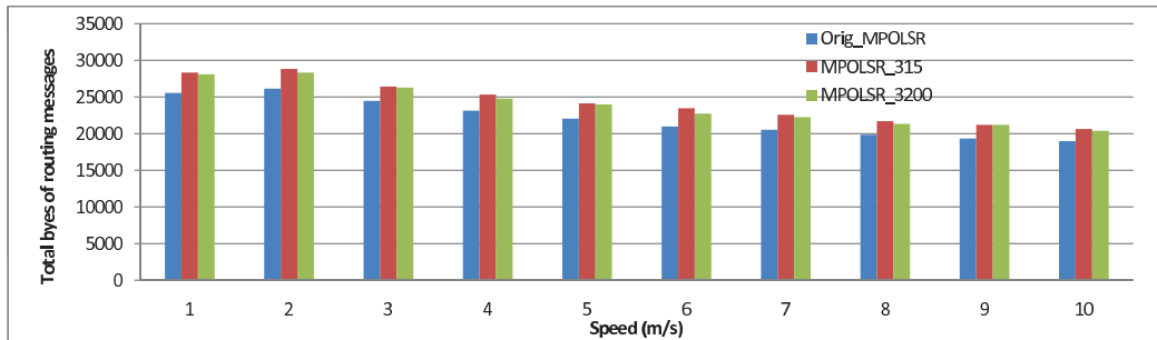
Figure 6.36: Total bytes of routing message
