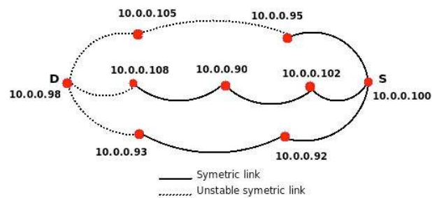
Figure 7.10: Quality of links in scenario 2: OLSR and MP-OLSR with 3 paths
