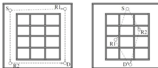
Figure 1.17: Experiment scenarios for video stream testbed with 4 nodes in the library building with topology line-of-sight (left) and behind the walls (right)
