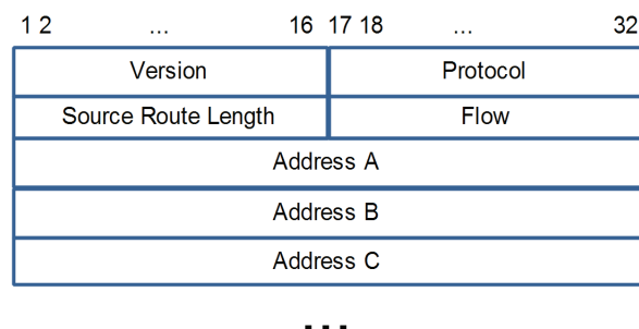
Figure 5.13: MP-OLSR header
