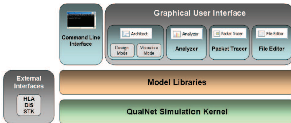
Figure 6.7: Qualnet Architecture
