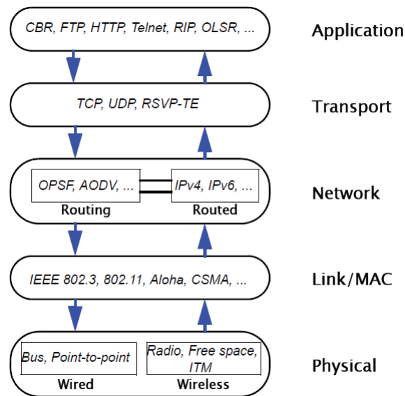
Figure 6.11: Qualnet Protocol Stack
