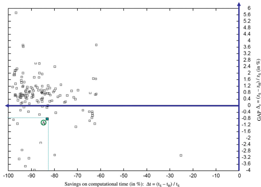
Fig. 4. Performance of the heuristic on L instances. The horizontal axis represents the relative gap in computational time \Delta_t between the heuristics and the solver. For example -50\% means that the heuristics is twice faster. The vertical axis represents the relative gap \Delta_z on the objective function. Each small square represents one of the 150 instances of families L1–L5. Let us consider the example of instance A: the savings on computational time is 82.5% while the objective function obtained with the heuristic is 1.8% better than the one obtained with the solver after 3 h of computation.
