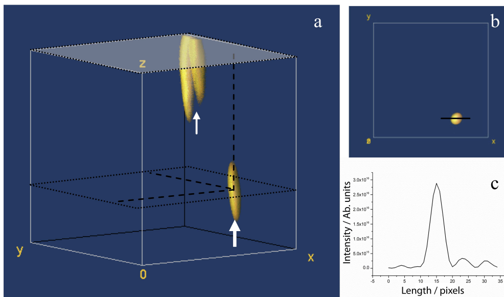
FIGURE 2.9: (a) 3D volume representations of scattered intensity isosurfaces, along with (b) XY plane section and (c) scattering intensity, showing the object to be diffraction-limited in size. In (a) the upper white plane corresponds to the electrode plane.
