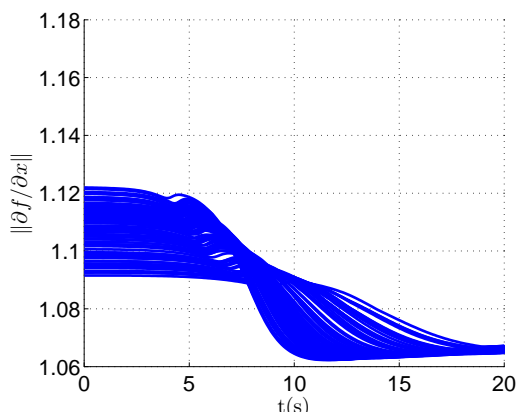
Figure E.1: Values of \|\mathbf{J}_f\|_2 at each instant for each of the 100 real trajectories
