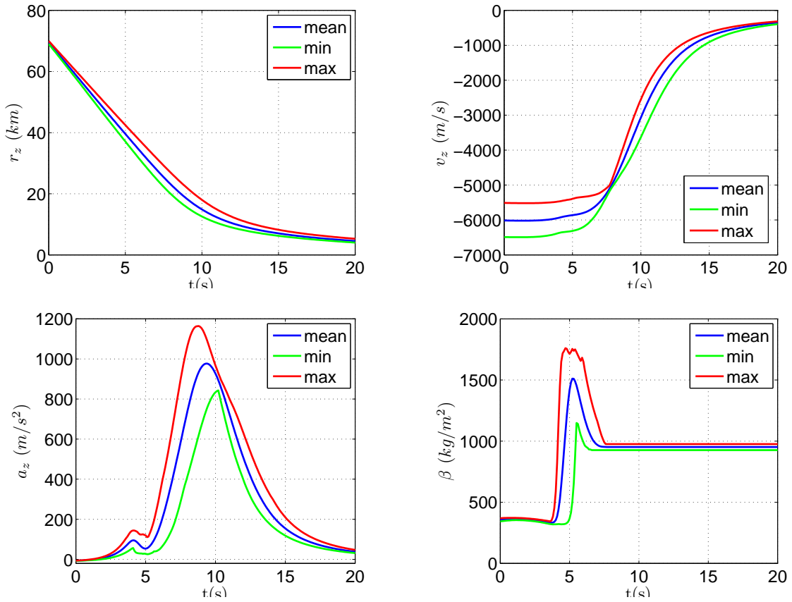
Figure 3.3: Evolutions of the position, velocity, acceleration and ballistic coefficient of one of the simulated trajectories
