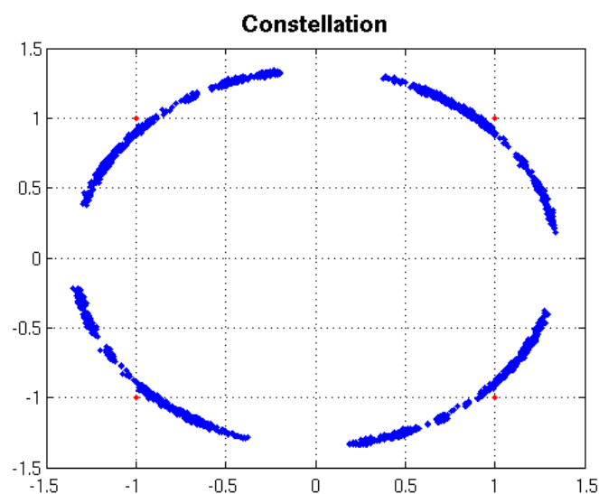
Figure III-24 : Constellation QPSK
