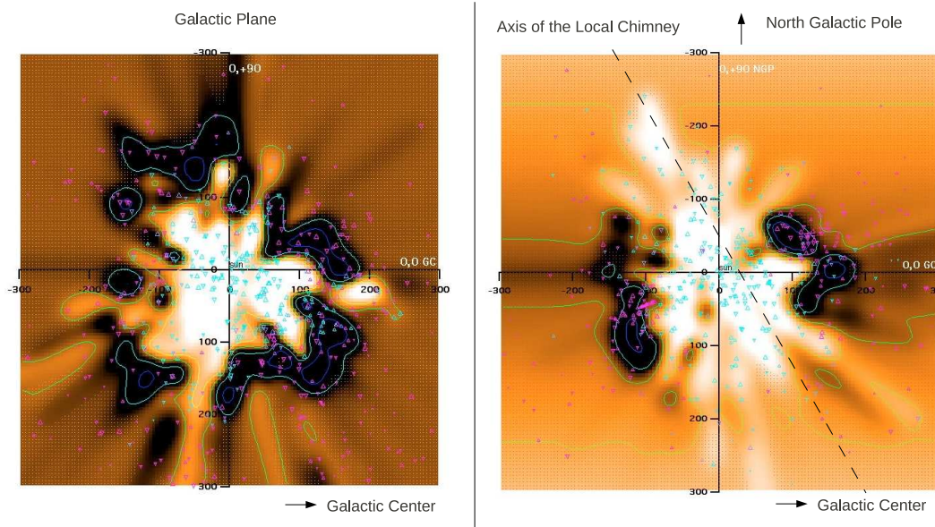
Figure 1.5: Plots of 3D spatial distribution of interstellar NaI absorption within 300 pc of the Sun as viewed in the Galactic plane projection (left) and in the meridian plane projection (right). White-to-dark shadings represents low-to-high values of the Na I volume density, which outline the edge of the Local Cavity. Figures adapted from Welsh et al. (2010) .
