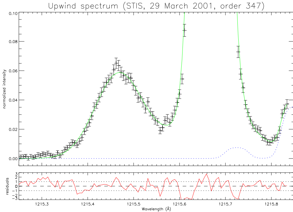
Figure 2.6: Fitting of STIS observations (29 March 2001) for the order 347. The blue dotted lines represent the contaminations by oxygen lines: 1306.029 Å (order 323) and 1302.168 Å (order 324), from left to right. This fit provides a line-shift of 22.4 \pm 0.4 km/s.
