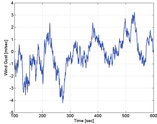
FIGURE 2.11: Dryden gust.
