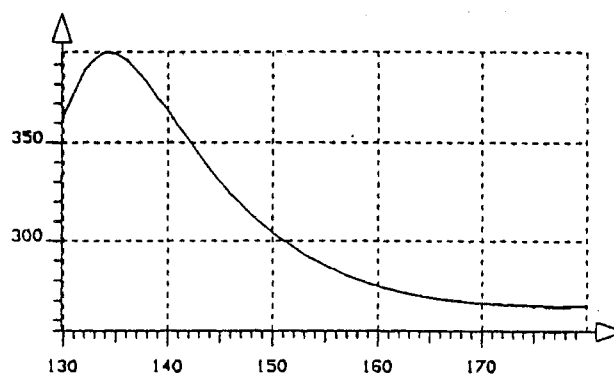
fig. III.34 : Tension aux bornes de la charge = f(\alpha)
