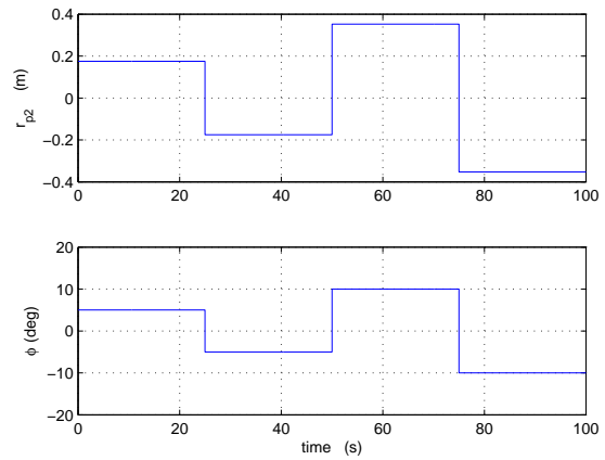
Figure 4.10: The roll angle is mainly controlled by the lateral translation of the movable mass.
