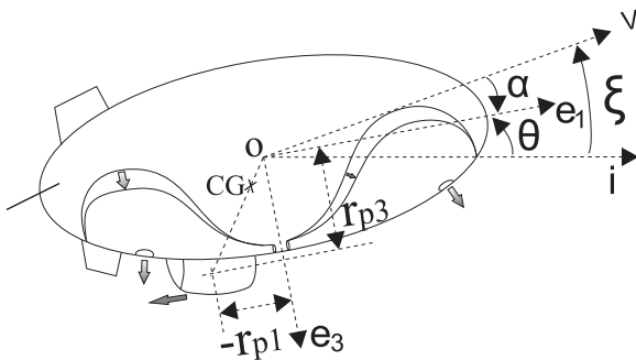
Figure 2.7: The Airship moves upwards and forward.
