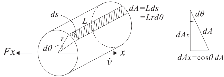
Figure 3.7: The added mass around a cylinder
