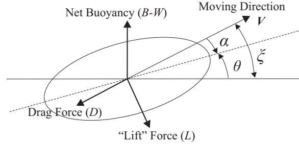
Figure 2.15: Ascent forces.
