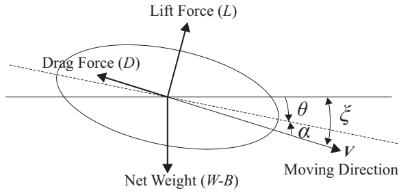
Figure 2.14: Descent forces.
