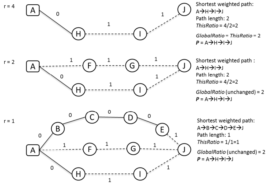
Figure 4.4 Illustration of the execution process of the path selection algorithm in Table 1 on a simple network.
