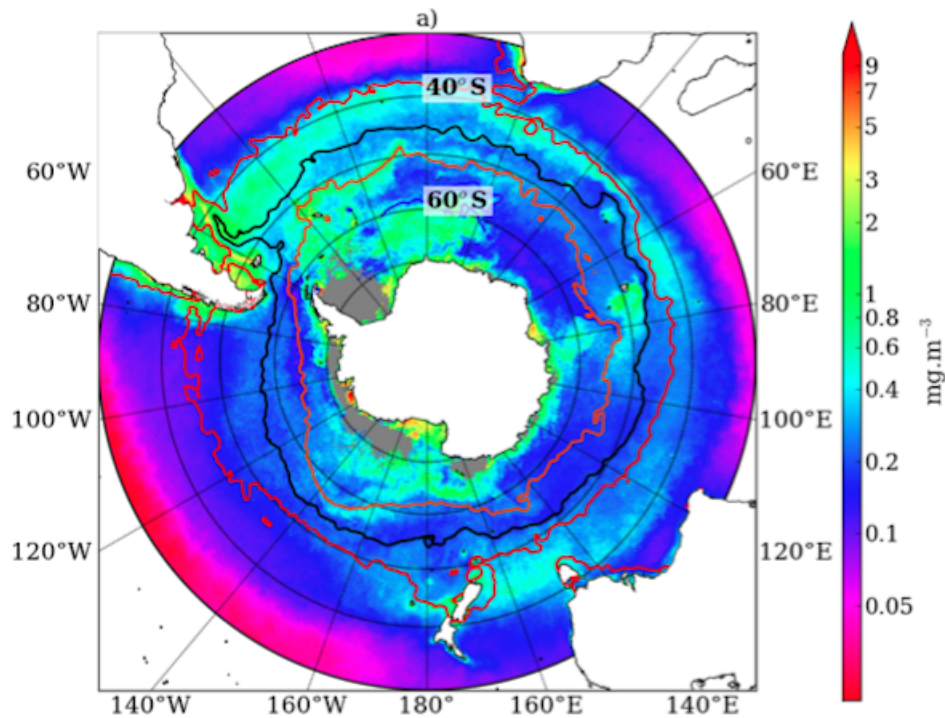
FIGURE 1.5: Spatial distribution of mean chlorophyll concentrations for the Southern Ocean south of 30°S for summer-January. Mean January (1998–2007) frontal positions calculated from MADT contours are shown for the STF (red), the SAF (black), the PF (orange) and the SACCF (blue). From Thomalla et al. [2011]
