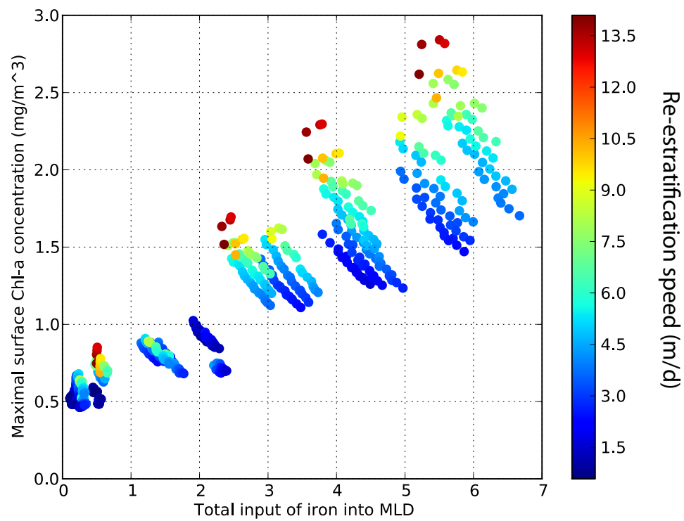
FIGURE 3.16: Maximal surface Chl concentration as a function of iron input into surface layer and Z_{mix} re-estratification speed (in color). Each circle stand for a modelled bloom.
