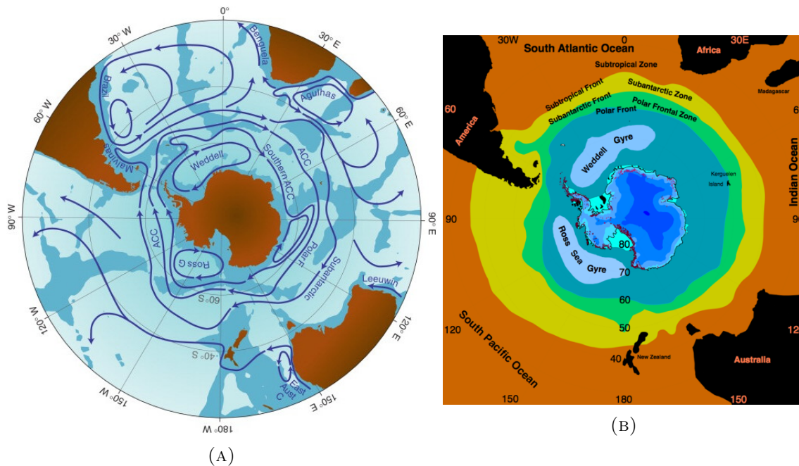
FIGURE 1.3: Left: A schematic view of the major ocean currents of the Southern Hemisphere oceans south of 20°S. Depths shallower than 3500m are shaded. C, current; G, gyre; F, front; ACC, Antarctic Circumpolar Current. From [Rintoul, 2009]. Right: A schematic view of the ocean frontal system in the Southern Ocean. From H.Grobe, Alfred Wegener Institute.
