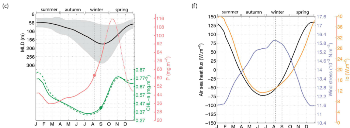
FIGURE 5.6: Mean of all seasonal cycle falling in (a-d) subtropical regime; (b-e) subantarctic regime; (c-f) ACC regime. Before taking the mean, all seasonal cycle are centred on their date of \text{Chl}^{\text{ML}}\text{-onset} . Panel (a-c) show the seasonal cycle of: (plain green) surface \text{Chl}_a ( \text{mg m}^{-3} ); (dashed green) associated surface carbon biomass ( \text{mg C} ); (pink) mixed-layer integrated chlorophyll, \text{Chl}^{\text{ML}} ( \text{mg m}^{-2} ); (black) mixed-layer depth from collocated in situ observation (m). Surface carbon biomass reads on the surface \text{Chl}_a axis, and has been multiplied by the following values to scale with \text{chl}_a : (a) 0.0124; (b) 0.0122; (c) 0.0098. Panel (d-f) show the seasonal cycle of: (black) air-sea heat flux ( \text{W m}^{-2} ); (purple) wind-stress ( \text{N m}^{-2} ); and (yellow) mixed-layer averaged irradiance ( \text{W m}^{-2} ). In panel (a-c) green dots indicates the median \text{Chl}^{\text{surf}}\text{-onset} date and pink dots the median \text{Chl}^{\text{ML}}\text{-onset} date detected by our automatic procedure (see text for details). \text{Chl}^{\text{ML}} is shown as a dotted line during the mixed-layer restratification phase to remind the reader that our estimate of \text{Chl}^{\text{ML}} is questionable during this period (see text for details). In panel (b), the black star on the \text{Chl}^{\text{ML}} curves denotes the time of \text{Chl}^{\text{surf}}\text{-onset} . \text{Chl}^{\text{surf}}\text{-onset} and \text{Chl}^{\text{ML}}\text{-onset} are reported on all panels by the vertical grey dashed lines
