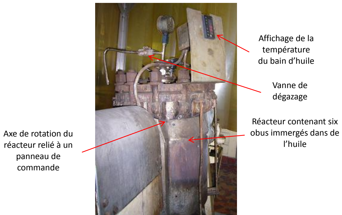
Figure III.1. Lessiveur rotatif
