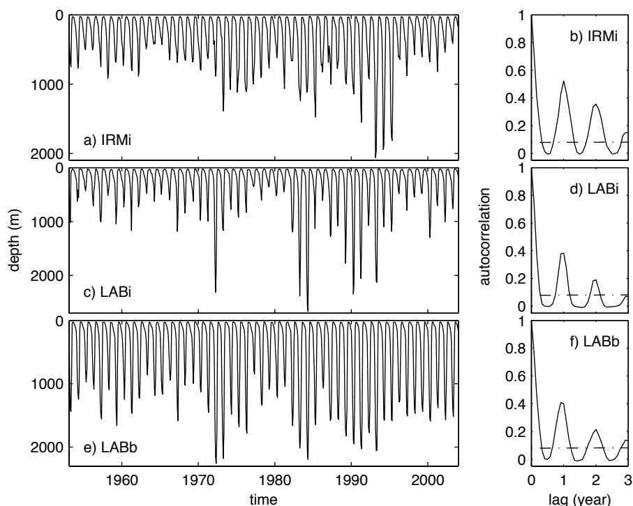
FIG. 3.28 – Thickness of the mixed layer in the regions of convection (left) and autocorrelation of the monthly anomalies (right). The dash-dotted lines indicate the 5% significance level for uncorrelated normal samples.
