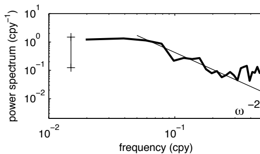
FIG. 4.14 – Power spectrum of PC1 of the MOC calculated with the multitaper method using three windows. The 95% confidence interval is given. Thin line indicates \omega^{-2} power law.
