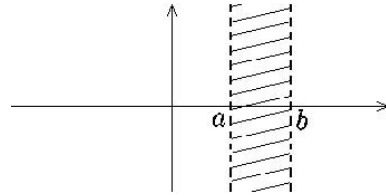
Figure 4.1: Fundamental strip < a, b > .
