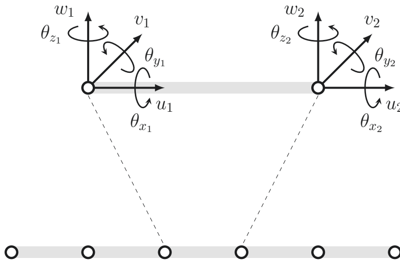
Figure 3.8: Illustration of the FEM mesh/element used to discretize the beam geometry.
