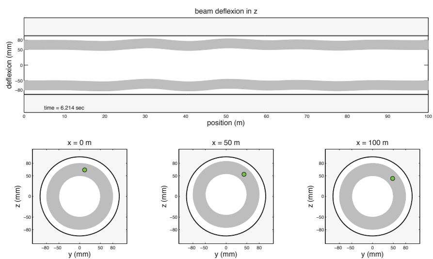
(c) t = 6.214 s
