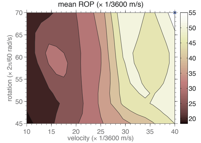
Fig. 36 Illustration of the contour plot of the mean rate of penetration function, for an “operating window” defined by 1/360 \text{ m/s} \leq V_0 \leq 1/90 \text{ m/s} and 3\pi/2 \text{ rad/s} \leq \Omega \leq 7\pi/3 \text{ rad/s} . The maximum is indicated with a blue cross in the upper right corner.
