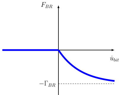
Fig. 7 Illustration of the function used to describe the reaction force on the drill-bit, due to the bit-rock interaction effects.
