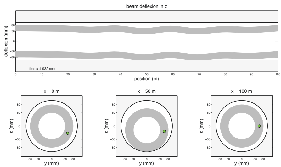
(b) t = 4.932 s
