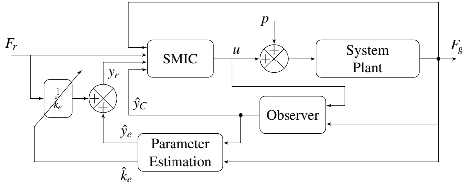
FIGURE 4.10: Diagram of the sliding-mode impedance control with force tracking.
