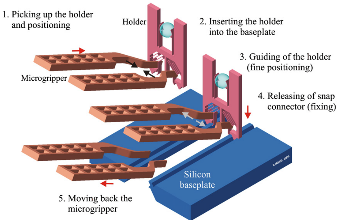
FIGURE 5.1: General concept of holder assembly based on the use of a robotic active microgripper as presented in [10].
