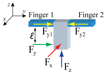
FIGURE 5.3: Perturbed grasp with each component of the contact force: F_x , F_y , and F_z .
