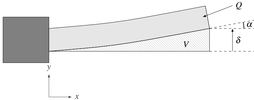
FIGURE 3.12: A top view of Figure 3.11 showing the displacement of the bimorph piezoelectric actuator and showing the output variables: the bending angle \alpha , the deflection \delta , the volume displacement V and the charge Q .
