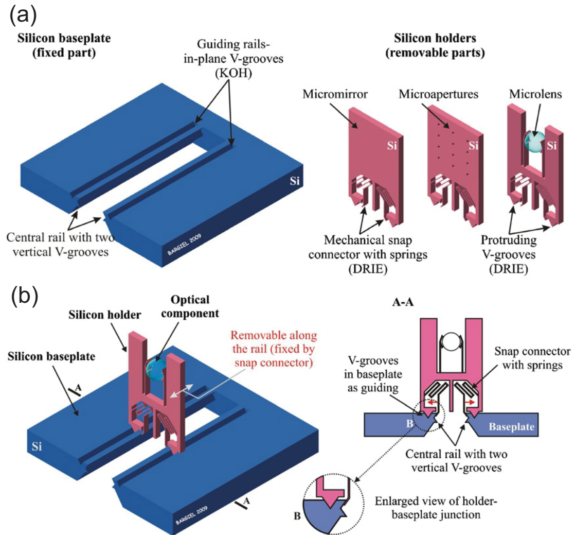
FIGURE 1.5: Individual components of the RFS-MOB and their assembly concept as presented in [10]: (a) details of the silicon bulk-micromachined baseplate and silicon holder (with the ball microlens as a micro-optical component), (b) holder assembled into the central rail of the silicon baseplate.
