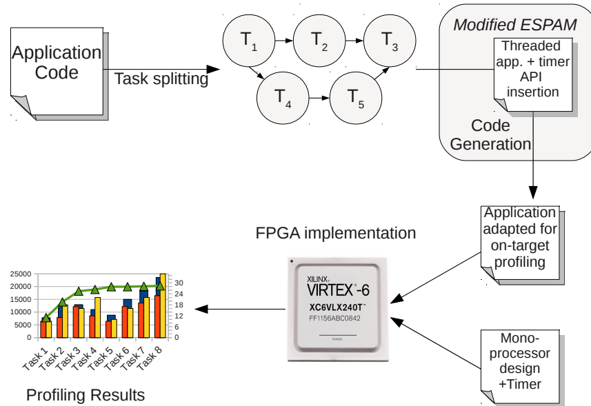
Figure 3.7: Flow of the profiling step.
