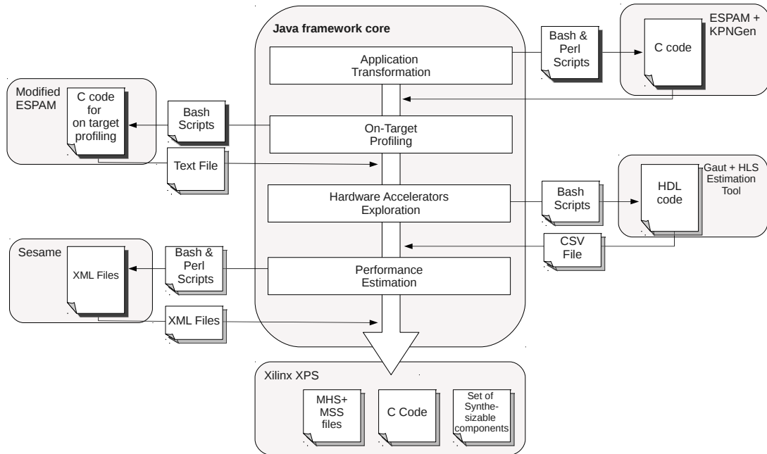
Figure 3.8: Technologies and formalisms used to interface with other tools.
