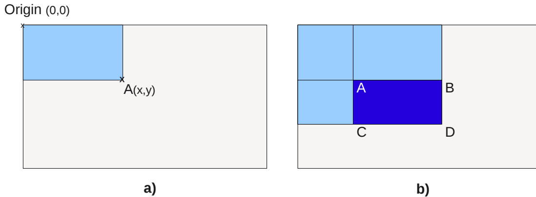
Figure 6.7: a) In integral image, the value of the pixel A is the sum of all the pixels in the colored rectangle. b) The computation of the rectangle defined by the pixels ABCD is given by the formula ((D - B) - C) + A .
