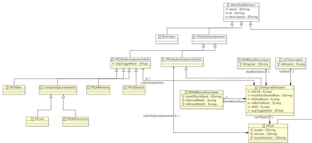
Figure 4.4: UML representation of the target FPGA metamodel.
