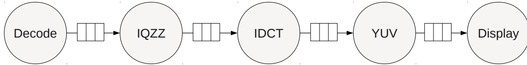
Figure 6.1: Representation of the Kahn Process Network of the implementation of the MJPEG decoder split in 5 tasks.
