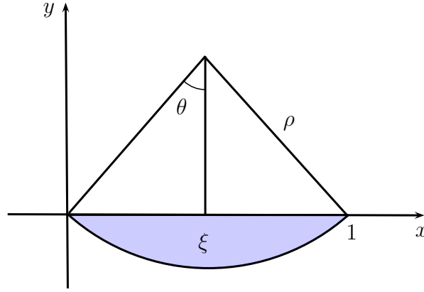
Figure 1.5: Projection of the geodesic joining the origin with (1, 0, \xi) in \mathbb{H} .
