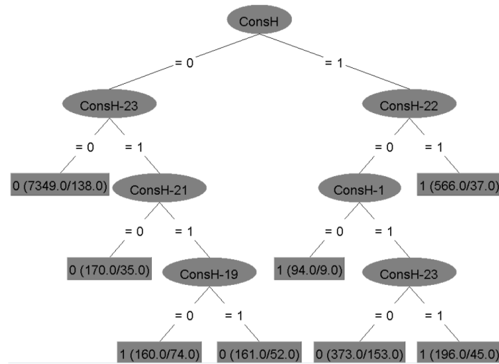
FIGURE 9.5 – The lighting prediction model (using DTL) in the house N° 925 of the IRISE database with only consumption information configuration for the oracle.
