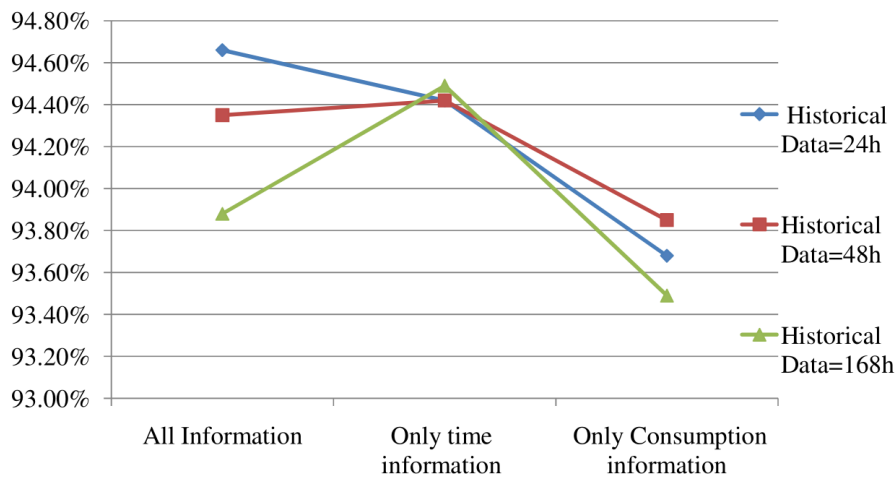
FIGURE 9.6 – The lighting prediction accuracy in the house N° 925 of the IRISE database using Decision Tree (C4.5 algorithm)
