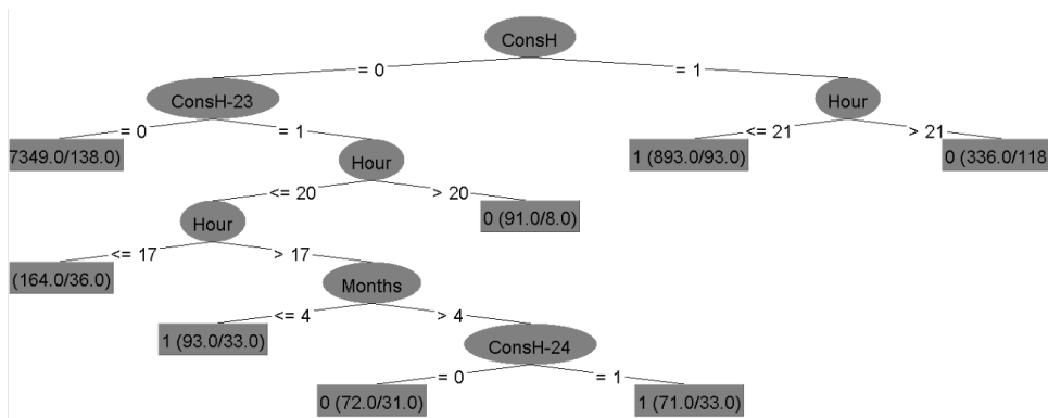
FIGURE 9.3 – The lighting prediction model (using DTL) in the house N° 925 of the IRISE database with all information configuration for the oracle.
