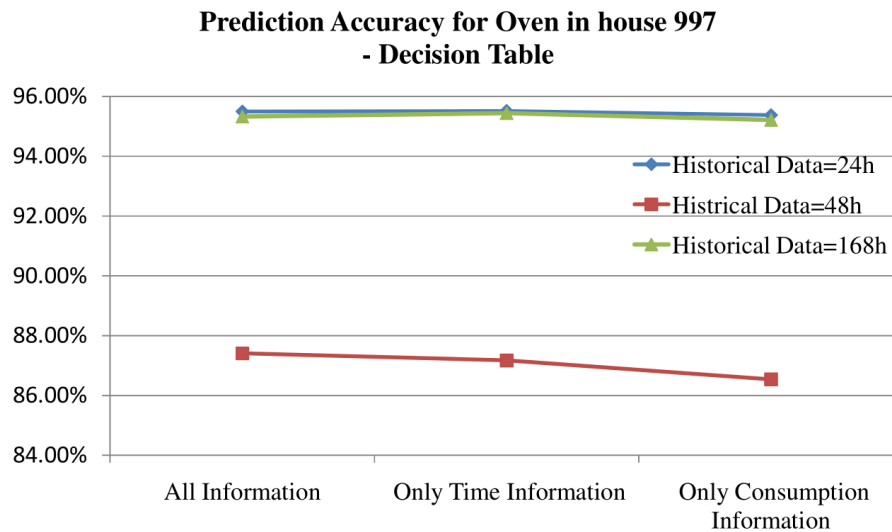
FIGURE 9.11 – The electric oven prediction accuracy in the house N° 997 of the IRISE database using Decision Table.
