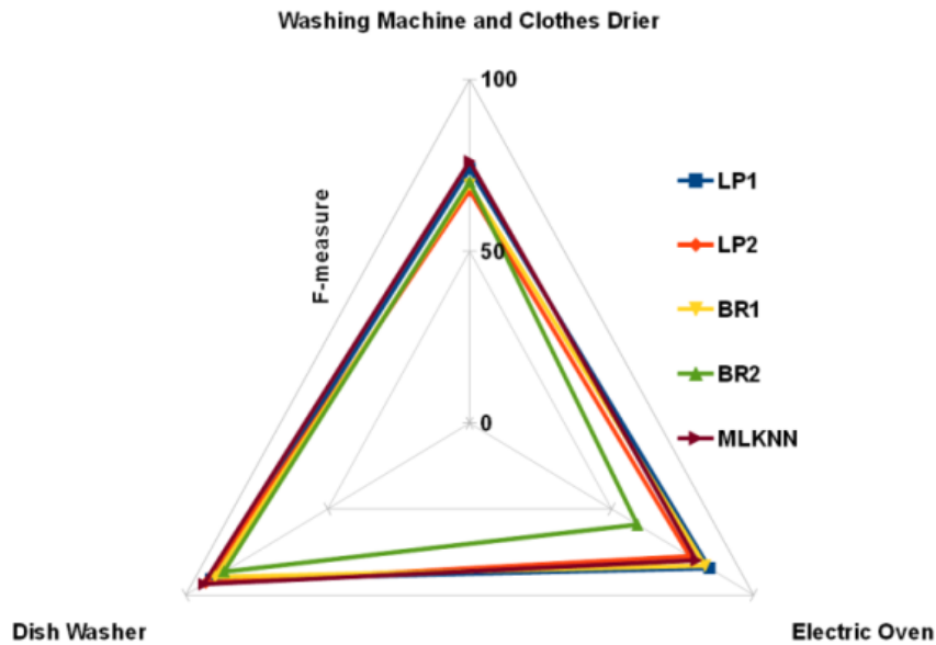
FIGURE 7.7 – Cat. 2 : Load identification performances considering some grouped appliances with a 10 minutes sampling time (acronyms in Section 7.3).
