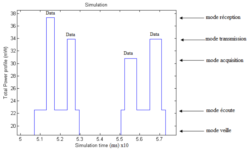
FIGURE 4.3 – Noeud utilisant le protocole sans acquittement
