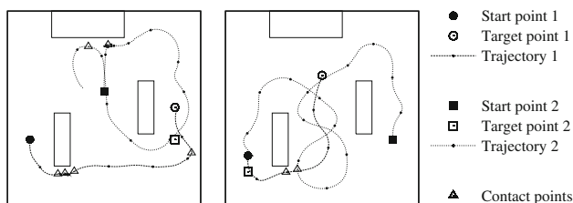
Fig. 11 Generalization performance of a 2-phase evolved controller using a free structure and four learning courses. The two figures show four trajectories obtained on test courses that are all different from the learning courses
