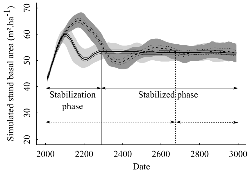
Figure 3: Simulated mean basal area and their 95% confidence intervals (bold and thick lines) and 95% prediction intervals (intervals) when individual demographic variability was considered (plain line, light grey) or not (dotted line, dark grey).
