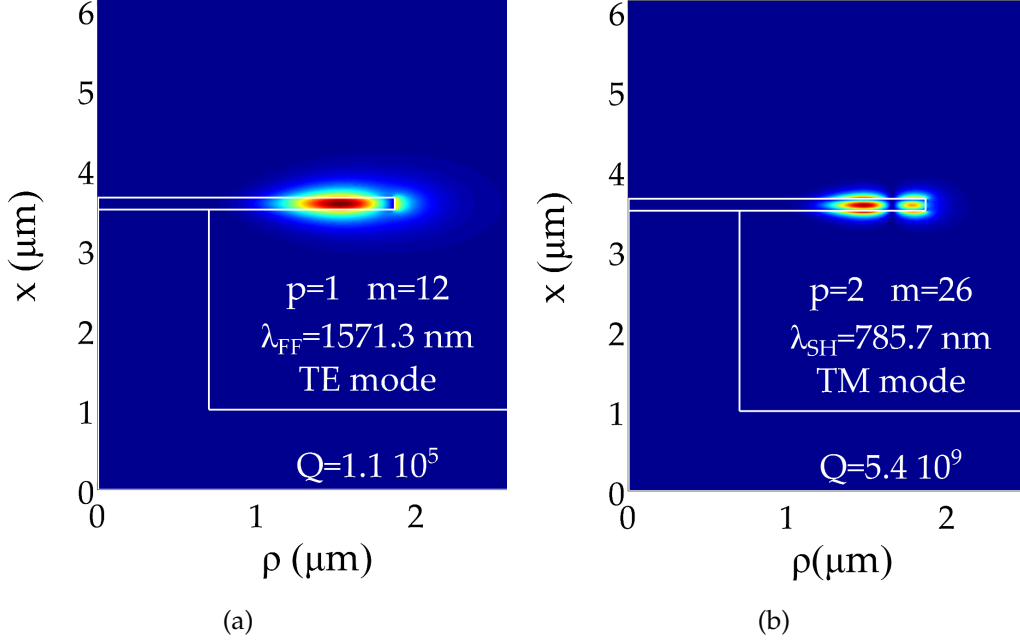
Figure 2.5: Transverse section of an Al 0.4 Ga 0.6 As suspended microdisk of radius R = 1.903 \mu\text{m} , height h = 155 nm and pedestal radius R_p = 0.5 \mu\text{m} , showing the 2D radial profile of the WGMs that are phase-matched and that conserve the energy, for the FF (a) and the SH (b) fields.
