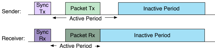
Figure 2.3: MAC protocol with common active periods
