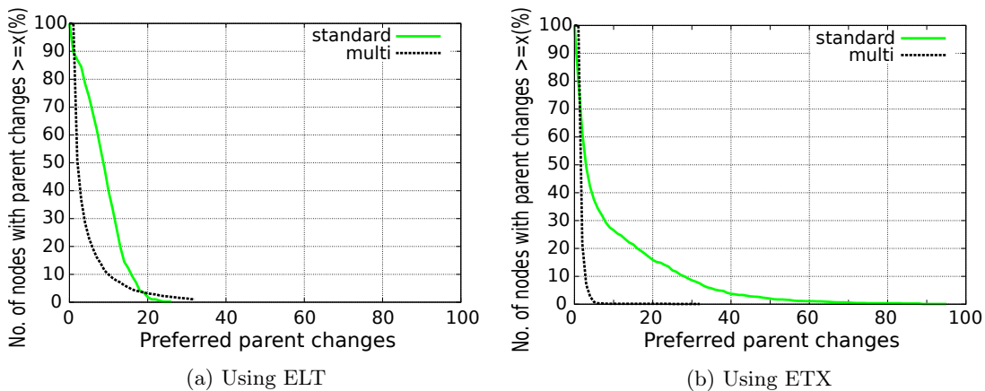
Figure 6.12: CCDF of the number of preferred parent changes during the whole simulation
