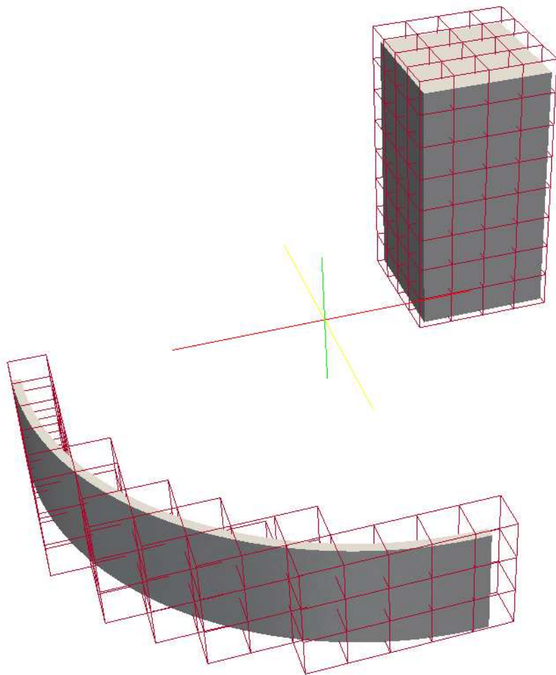
FIGURE C.1: Space partitioning for the sound barrier at the 4 th level.
