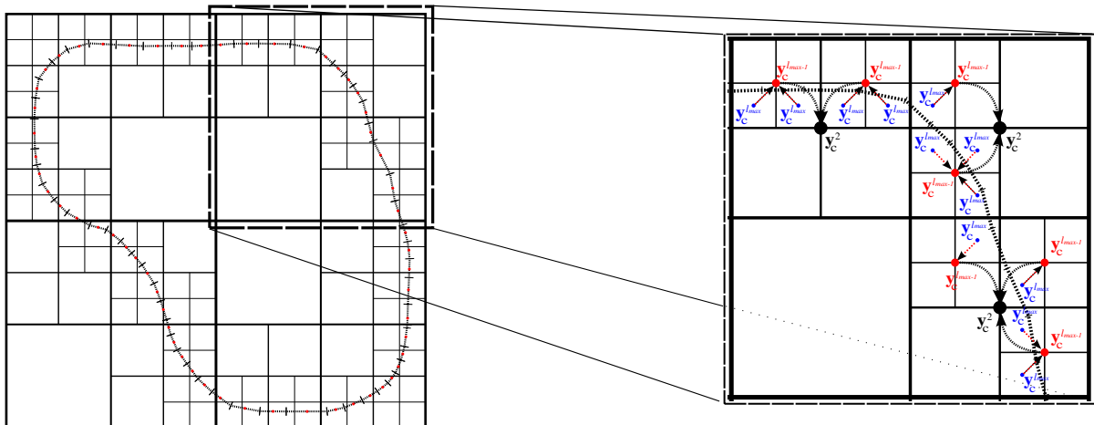
FIGURE 3.6: During the Moment to Moment (M2M) step, the expansion coefficients of children at a level l are translated towards the expansion center of their parents \mathbf{y}_c^{l-1} and summed. This step is performed until the level l = 3 .
