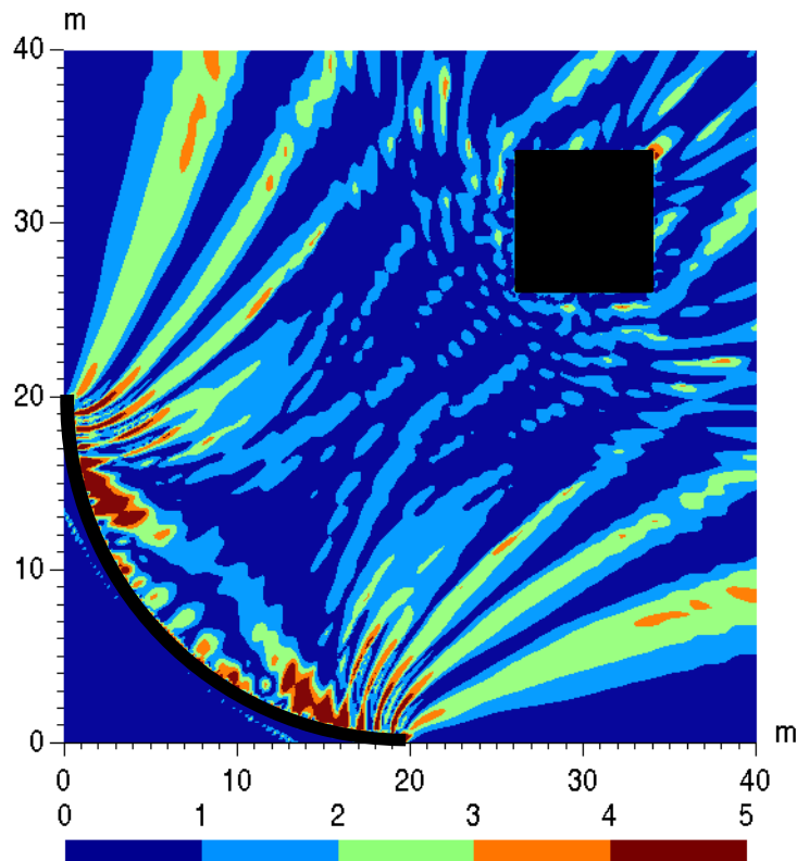
FIGURE 5.5: Differences (in dB) between the noise maps obtained with Micado3D and the FMBEM for the frequency range (170-190 Hz). The sound barrier and the building are displayed in black (top view).
