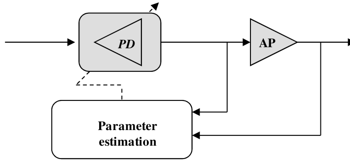
Figure 2.12 – Direct learning architecture
