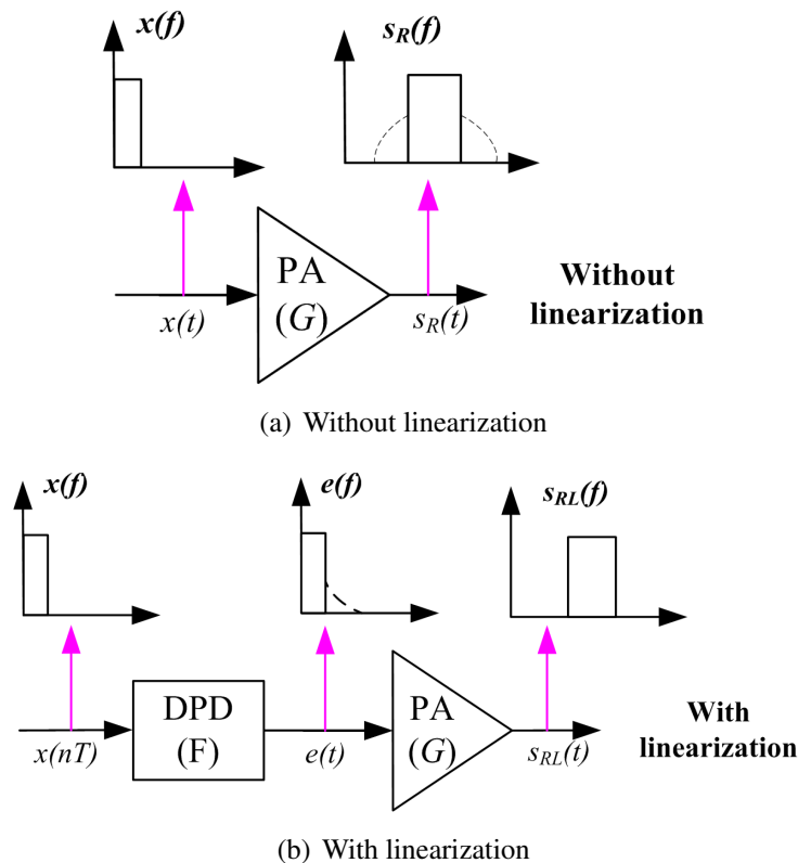
Figure 2.14 – Spectrum of Baseband DPD
