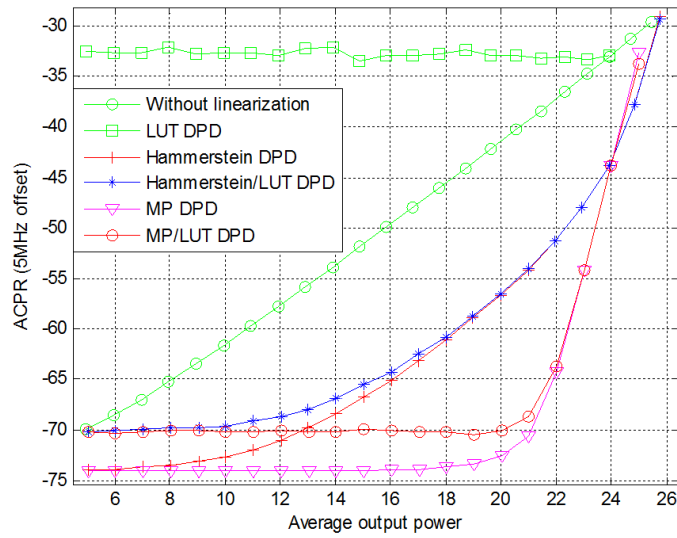
Figure 3.20 – Simulated ACPR
