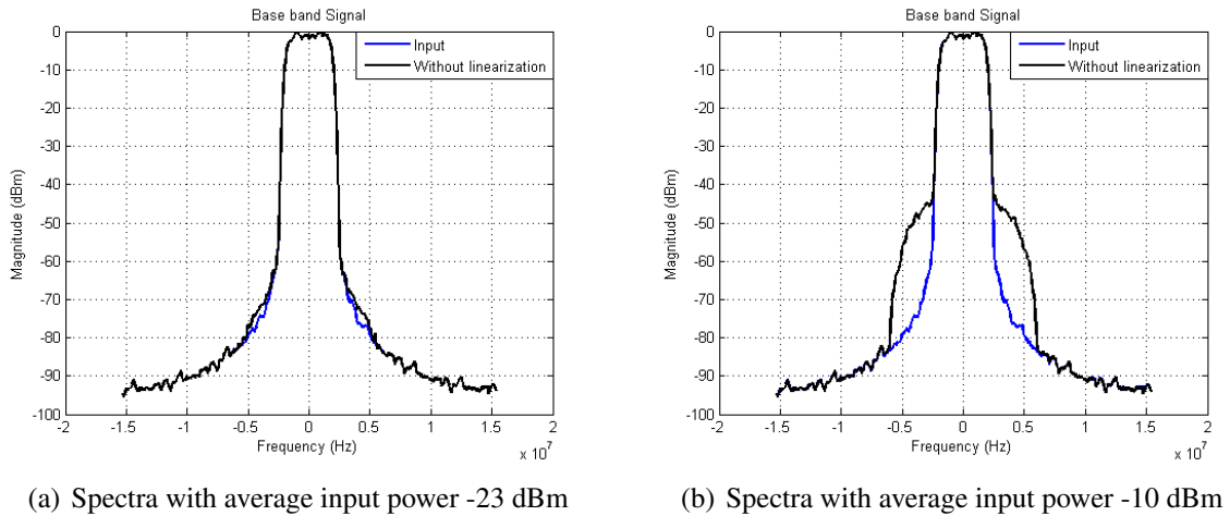
Figure 3.5 – Nonlinearity presented by spectral regrowth
