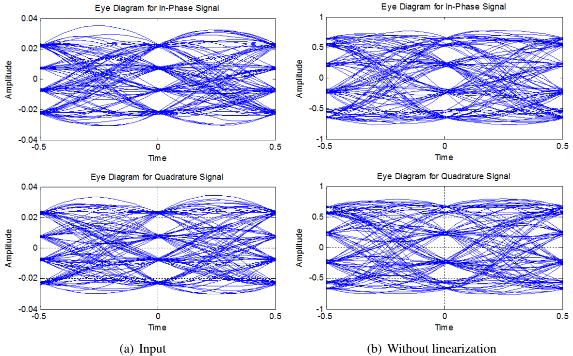
Figure 4.18 – Eyediagrams with average input power of -11 dBm
