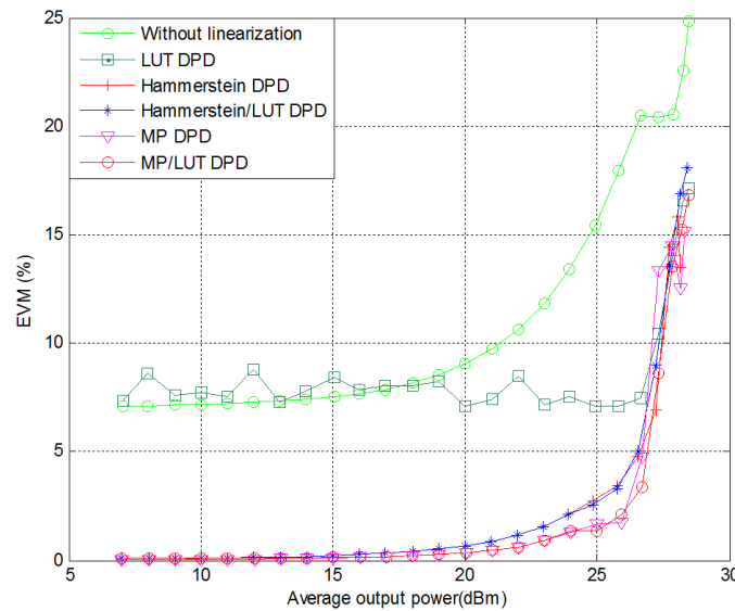
Figure 3.21 – Simulated EVM
