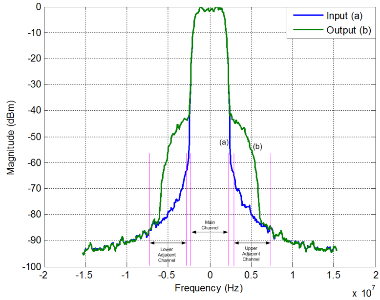
Figure 1.13 – Spectral regrowth
