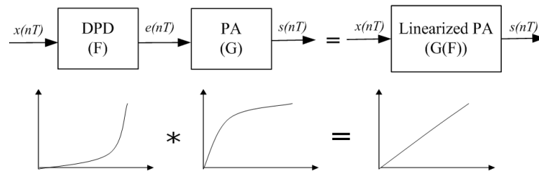
Figure 2.4 – Principle of Predistortion
