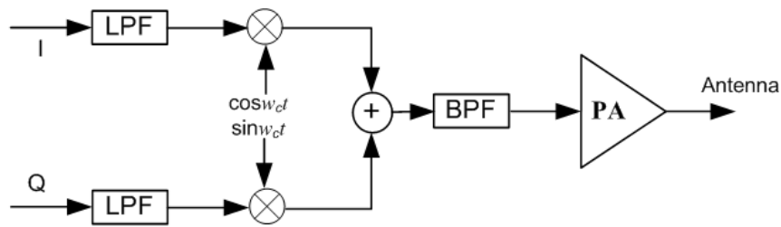
Figure 1.6 – Homodyne Tx
