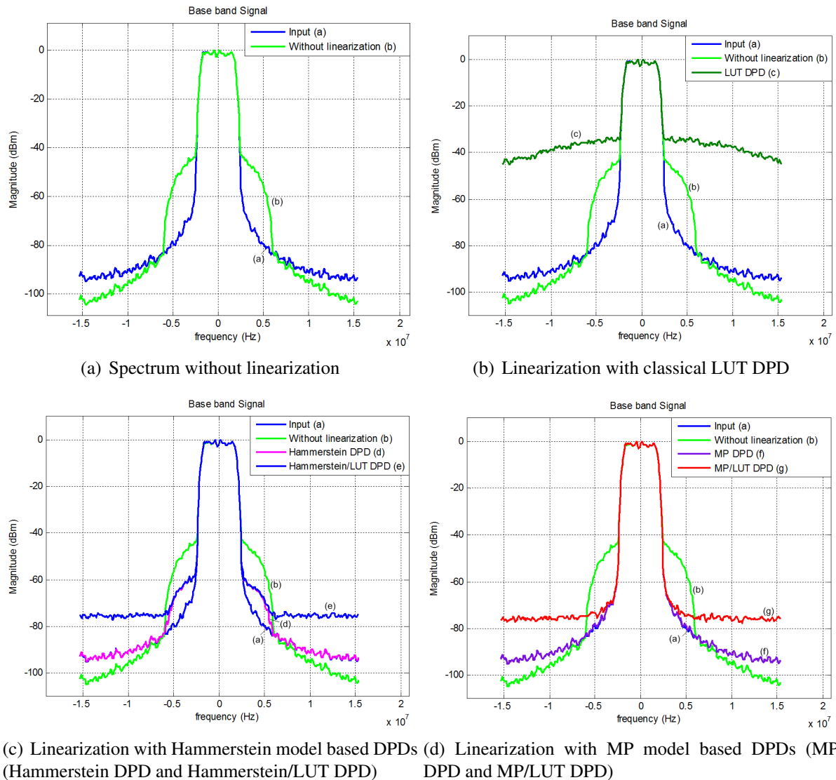
Figure 3.17 – Spectrum
