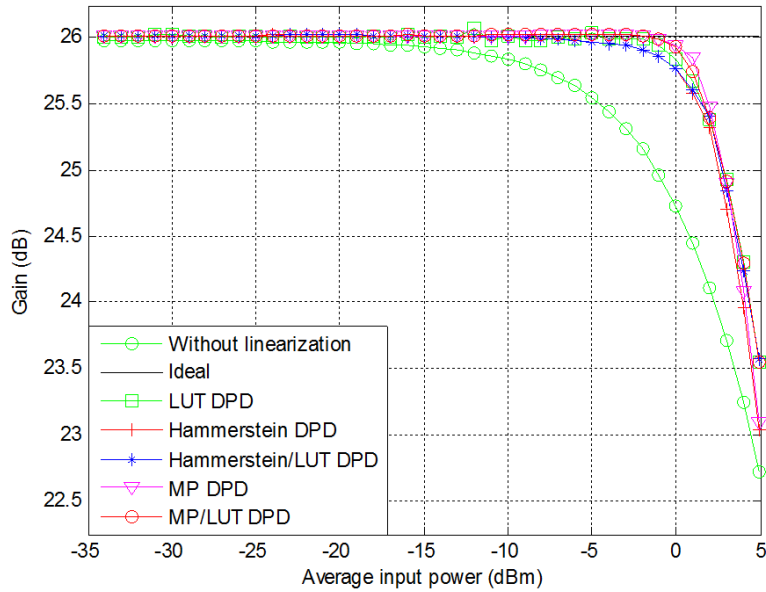
Figure 3.16 – Gain
