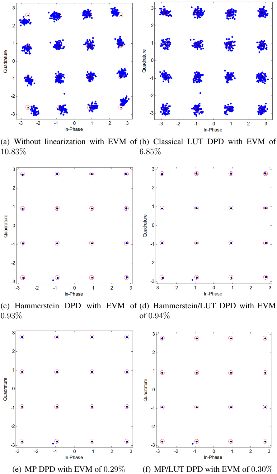
Figure 3.18 – Constellations with average input power -4 dBm
