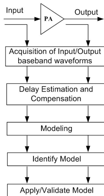
Figure 2.5 – Modeling procedure
