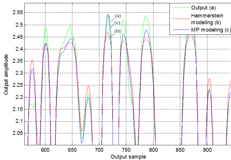
Figure 4.14 – PA modeling
