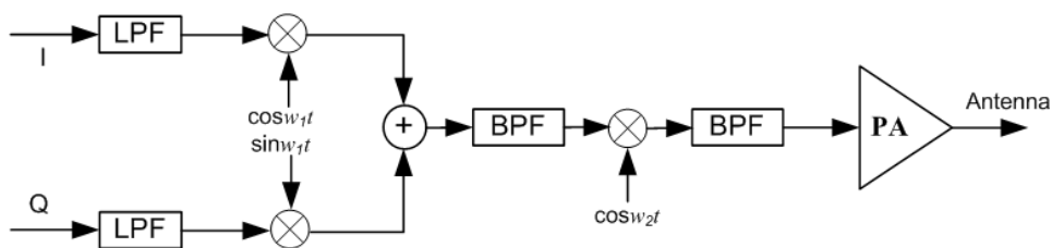
Figure 1.7 – Heterodyne Tx
