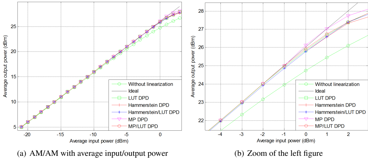
Figure 3.15 – AM/AM with average input/output power
