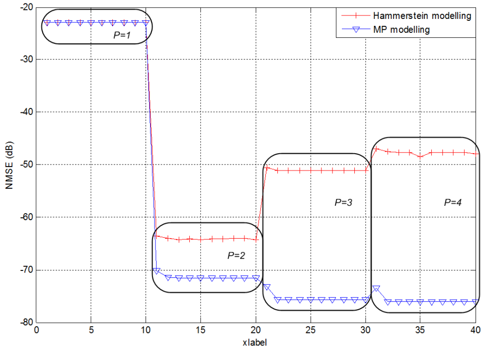
Figure 3.9 – Effect of number of coefficient on the performance of NMSE with average input power -10 dBm in the linear region
