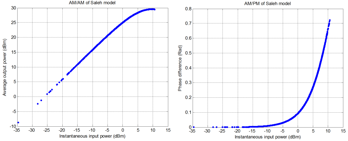
(a) AM/AM characteristic of the Saleh model
