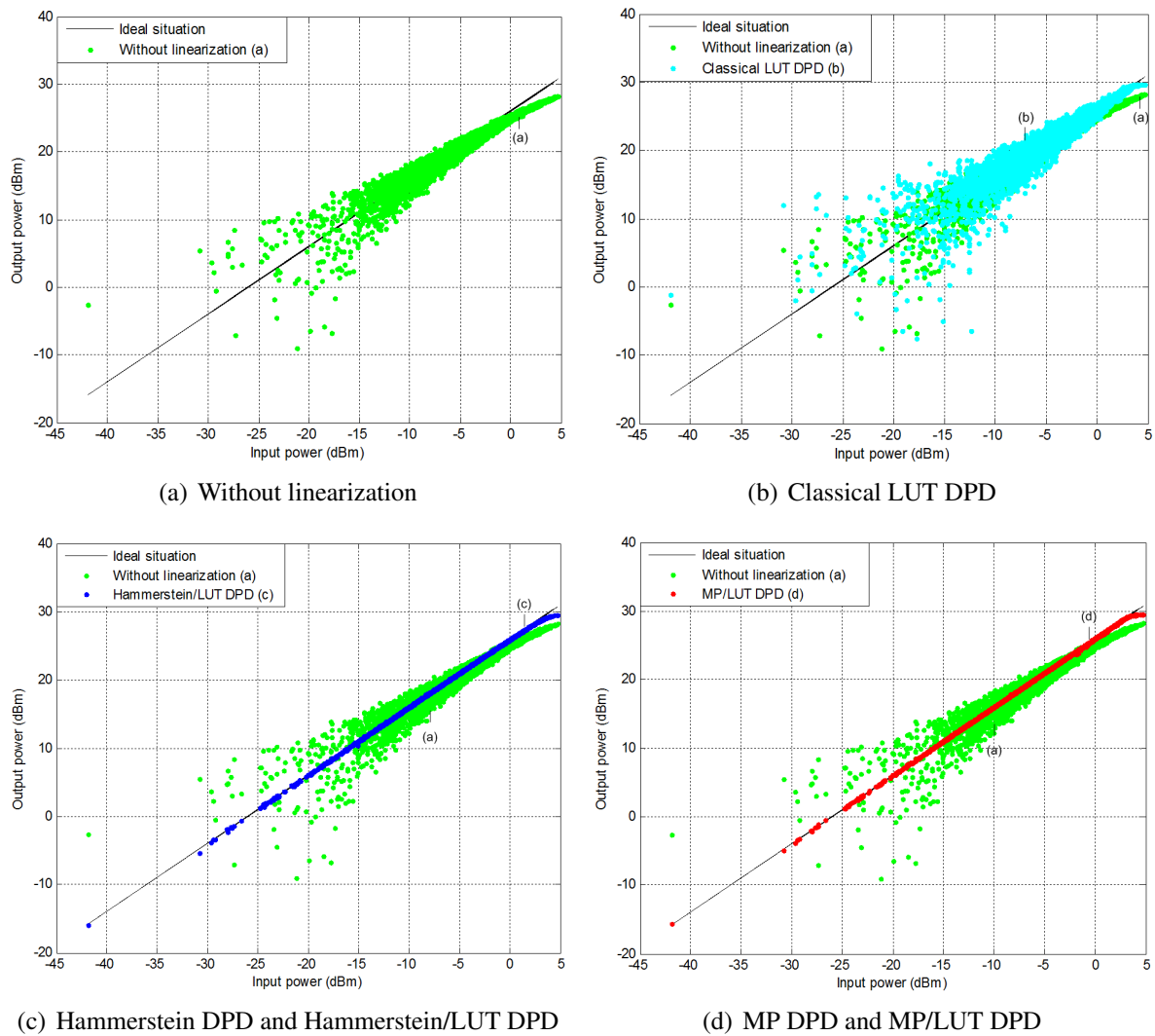
Figure 3.13 – AM/AM
