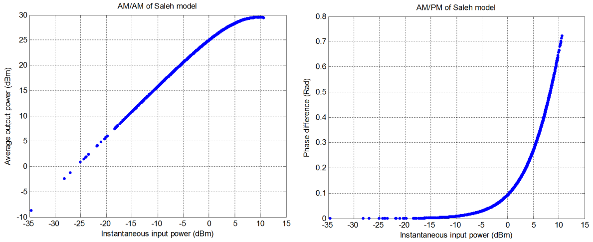
(a) AM/AM characteristic of the Saleh model
